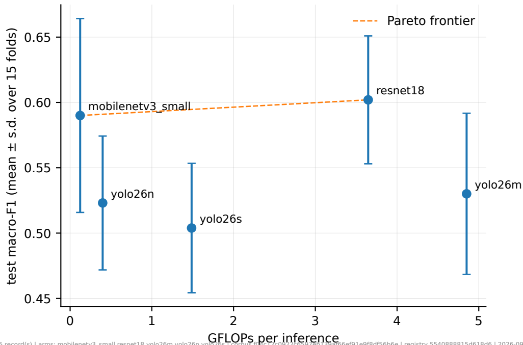
Accuracy against computational cost
