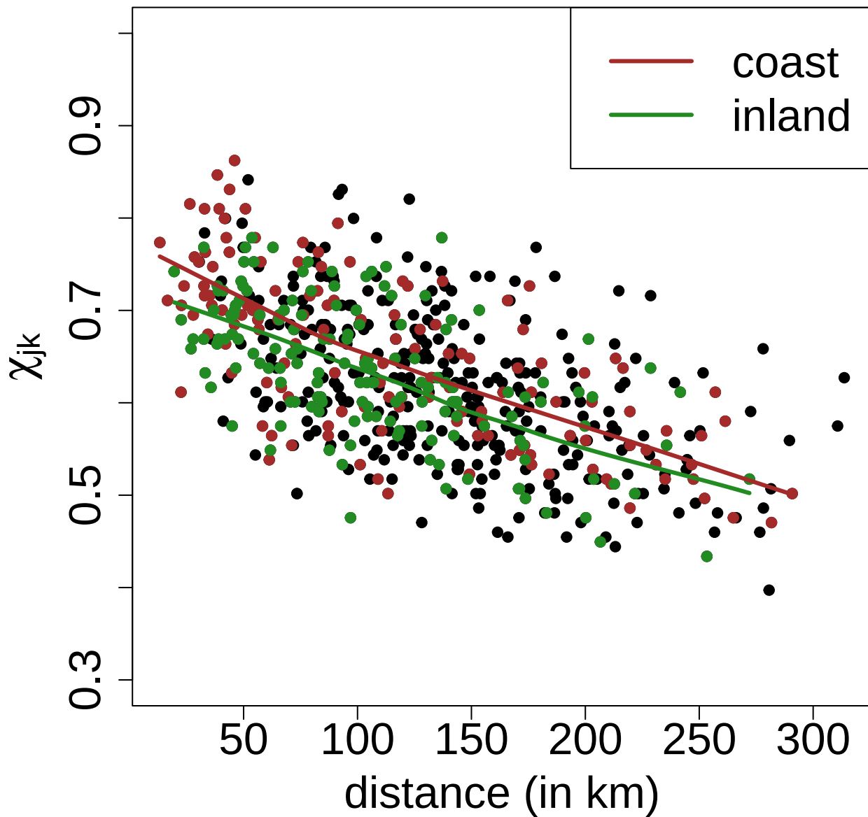
Tail dependence coefficients \chi_{jk}
