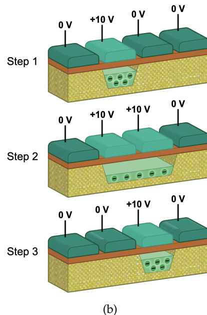
Figure 7: Panel (a): Schematic of a section of a CCD pixel with four electrodes. The channel stop prevents charge leakage from one pixel column to another. Charges are stored in a buried channel separated from the surface by an insulator. Panel (b): Charges are moved across a pixel through clocking. Images courtesy of Teledyne Imaging.
