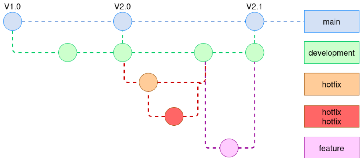
Figure 3: A fairly typical workflow for a software project.
