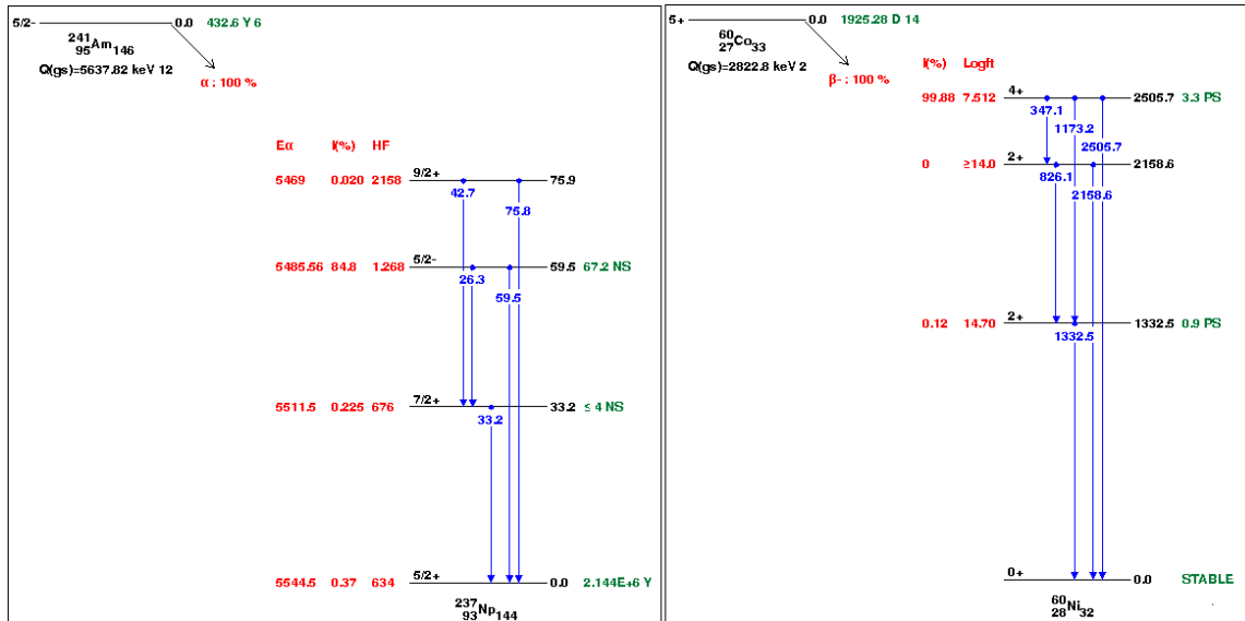
Figure 16: Left: the decay scheme of ^{241}\text{Am} to ^{237}\text{Np} showing the 60 keV transition. Right: The decay scheme of ^{60}\text{Co} to ^{60}\text{Ni} , showing the prompt cascade of the 1173 and 1332 keV transitions. Images are modified from Brookhaven National Laboratory.
