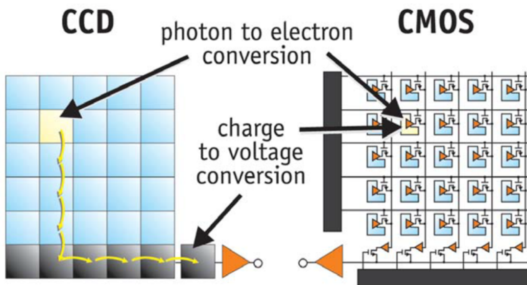
Figure 8: A cartoon demonstrating the charge-to-voltage conversion process for CCDs and CMOS detectors. Image courtesy of Stefan Meroli/CERN .
