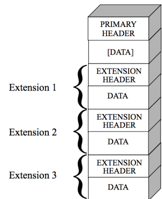
Figure 12: The building blocks of a FITS file. Image courtesy of the Space Telescope Science Institute.
