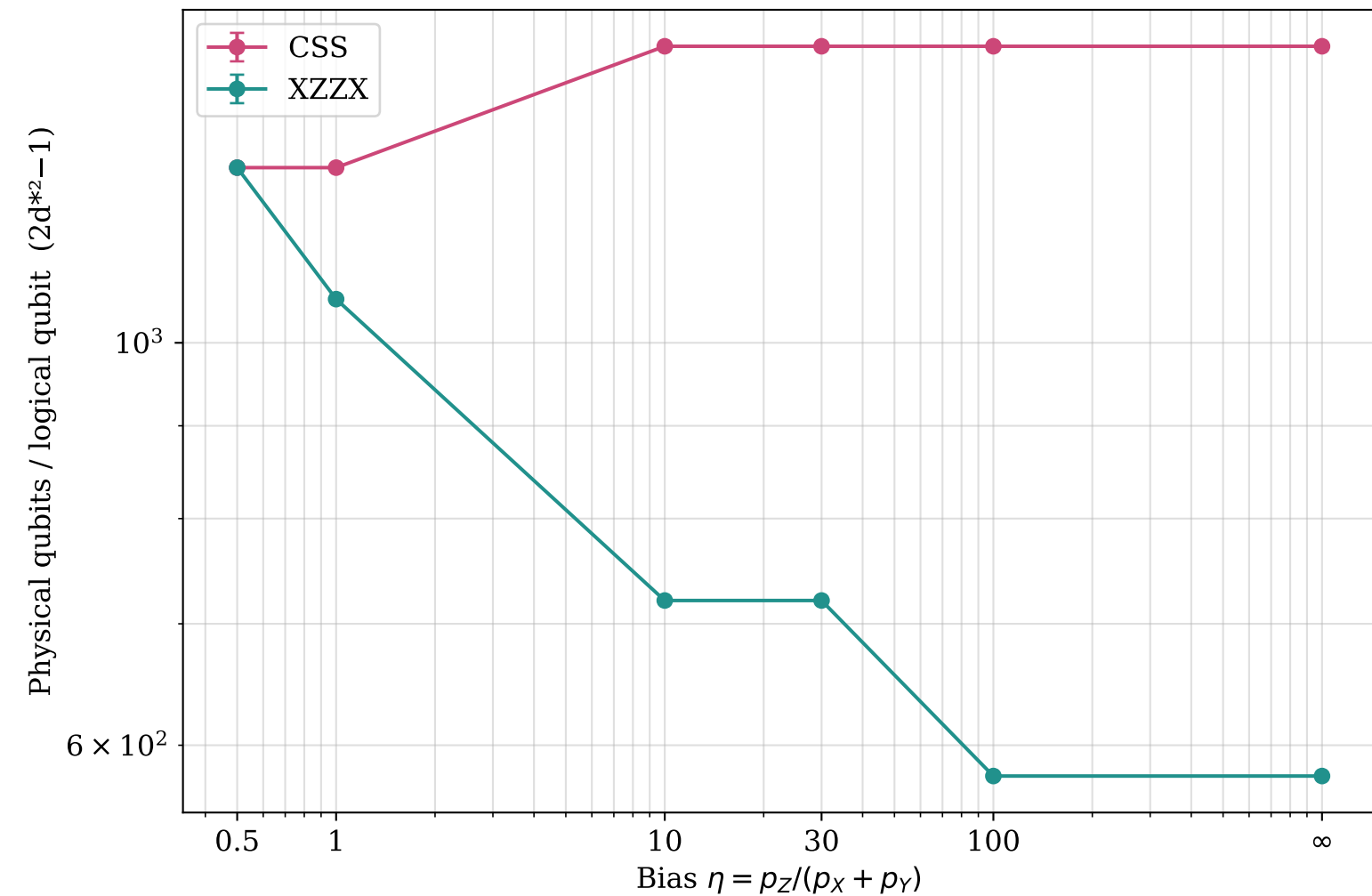
Physical-qubit cost vs bias (target per-cycle \varepsilon=1\text{e-}12 , physical p=0.001 ; memory only, square codes)
