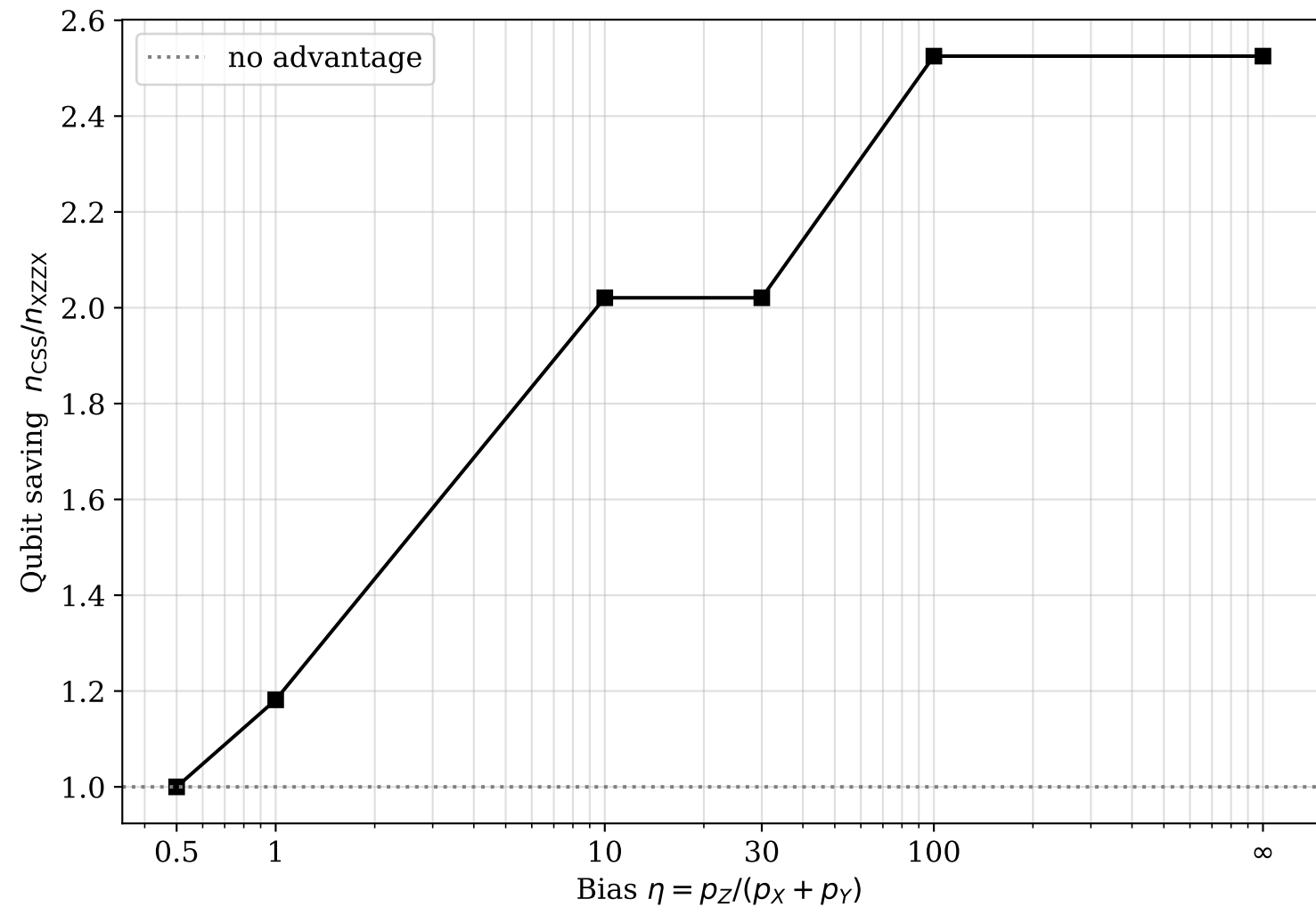
Physical-qubit cost vs bias (target per-cycle \varepsilon=1\text{e-}12 , physical p=0.001 ; memory only, square codes)
