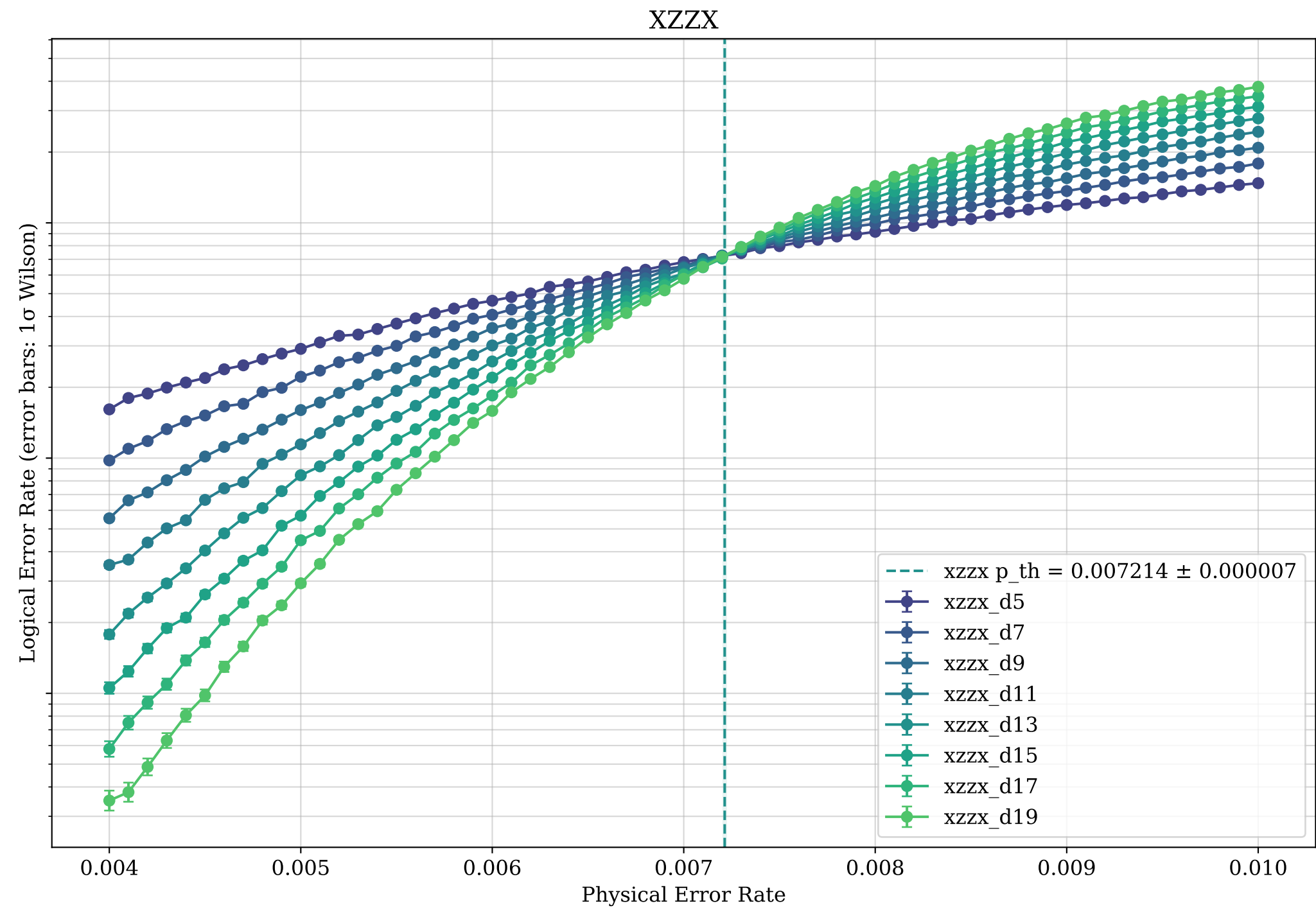
Rotated CSS Surface Code vs XZZX Code Simulation Results with \eta = 0.5
