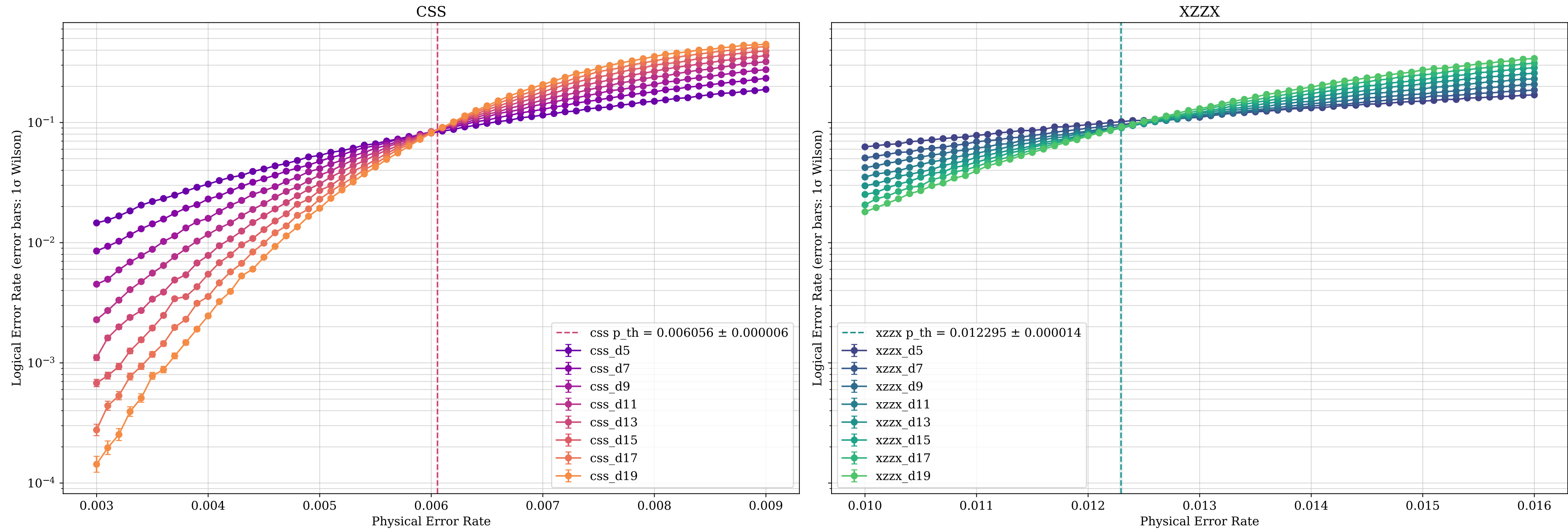
Rotated CSS Surface Code vs XZZX Code Simulation Results with \eta = 10
