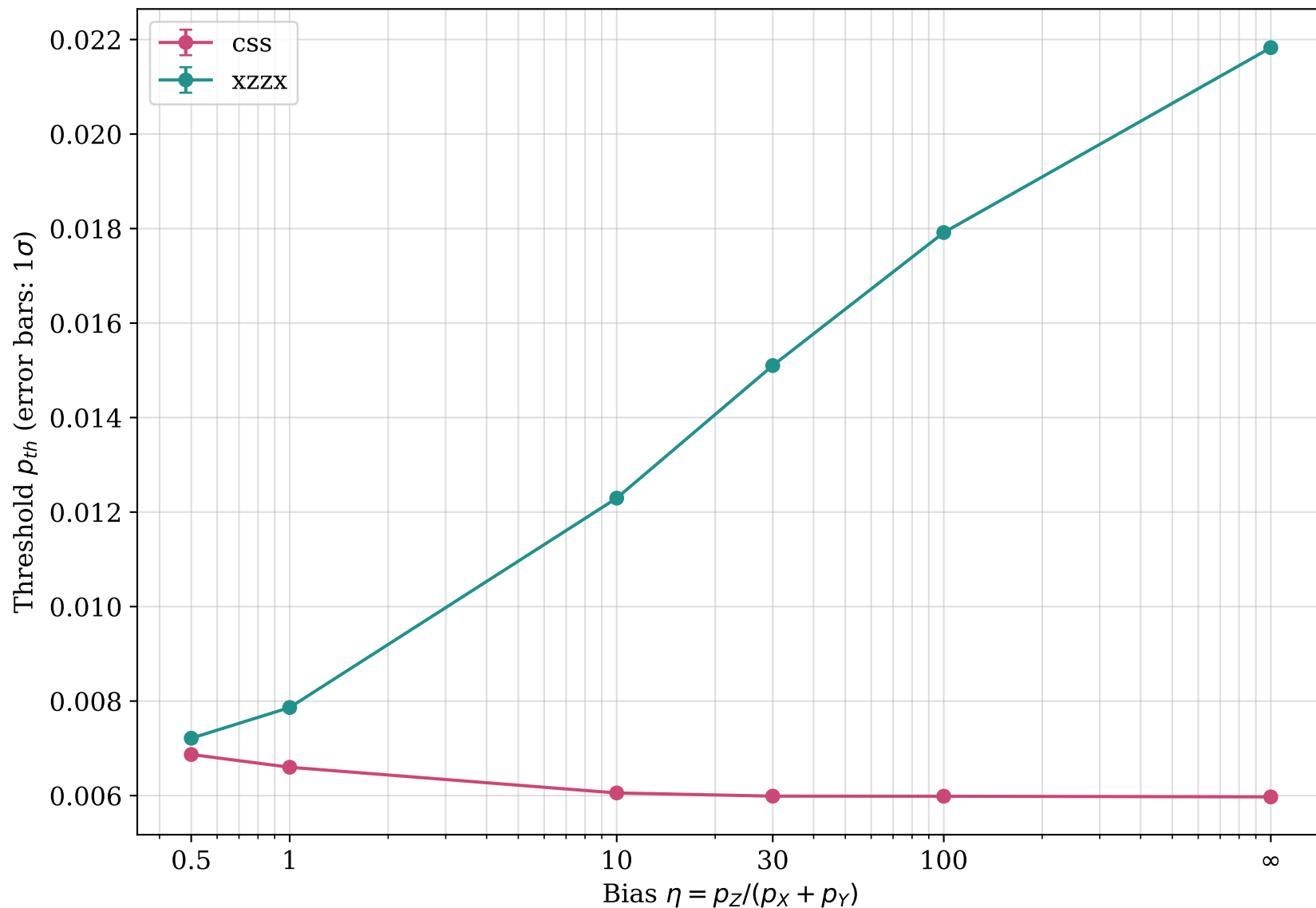
Threshold vs bias: Rotated CSS Surface Code vs XZZX Code
