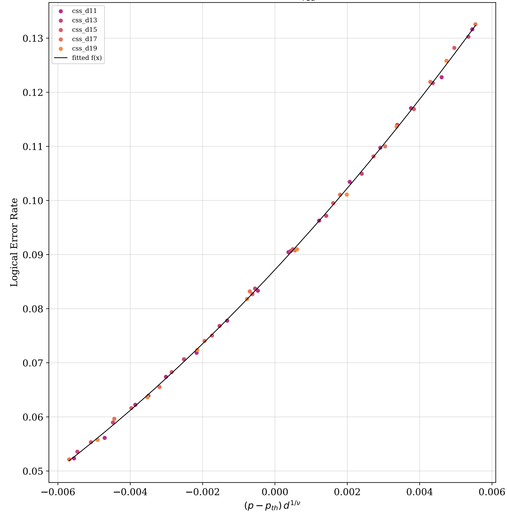
FSS data collapse ( \eta = 10 )
