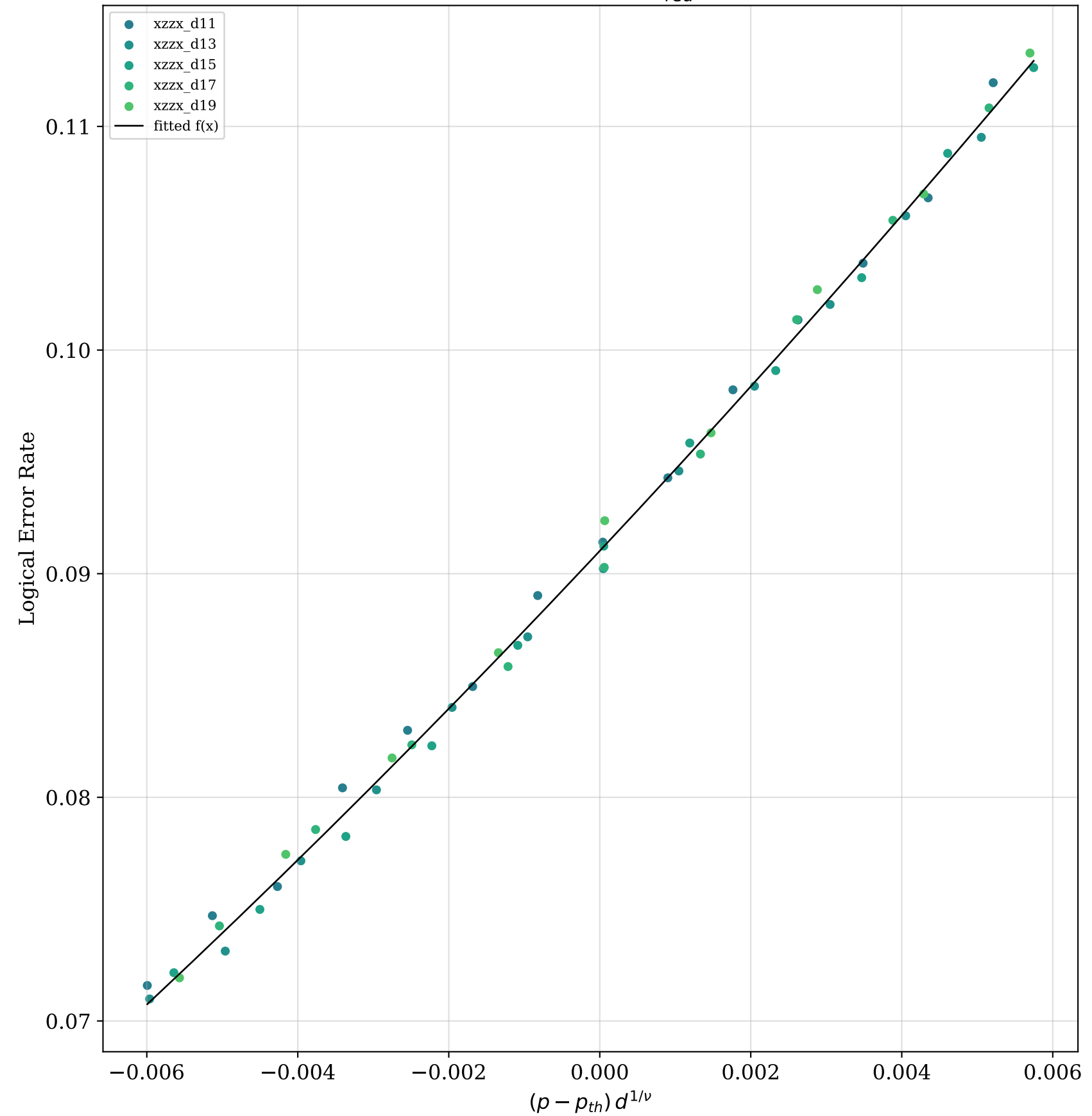
FSS data collapse ( \eta = 10 )
