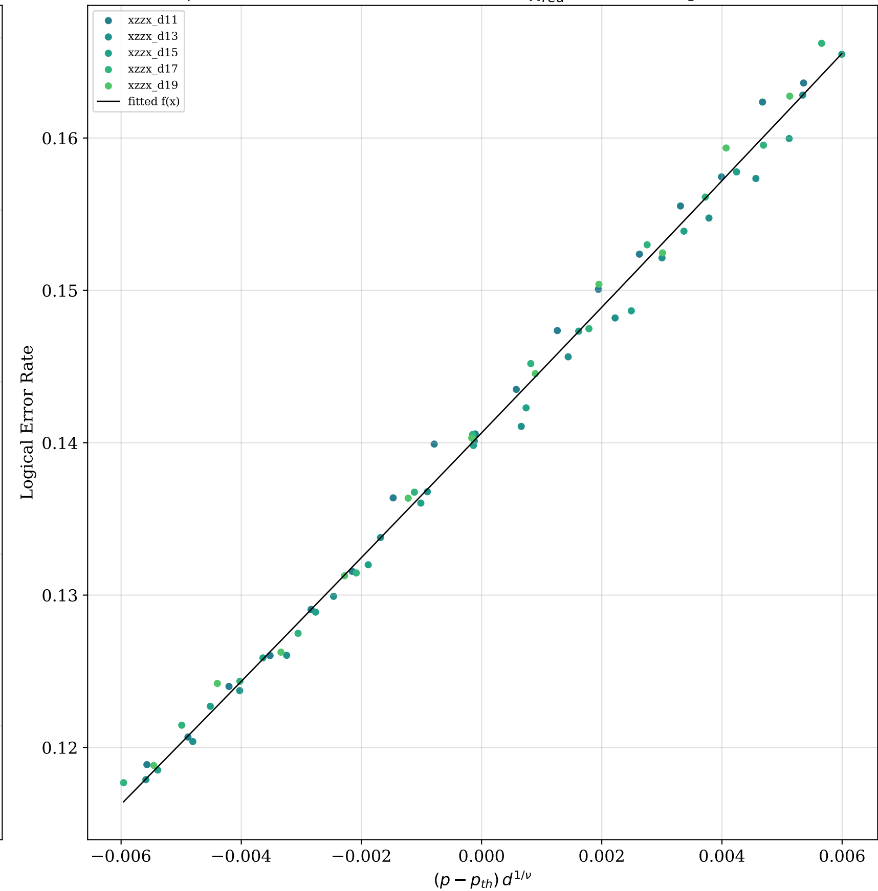
FSS data collapse ( \eta = 100 )
