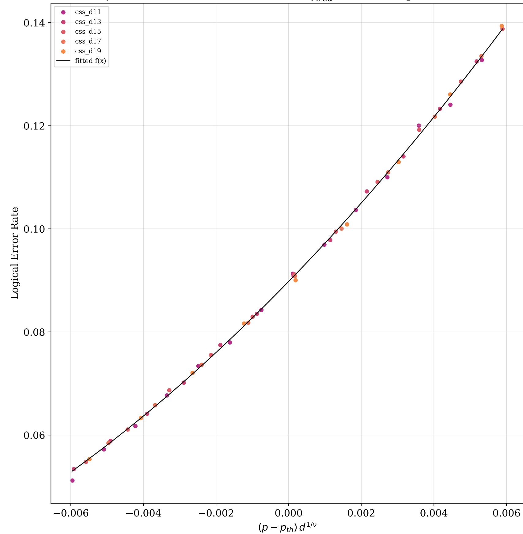
FSS data collapse ( \eta = 100 )
