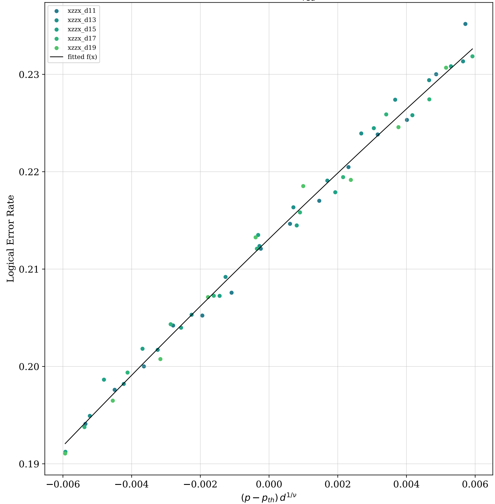
FSS data collapse ( \eta = \text{inf} )
