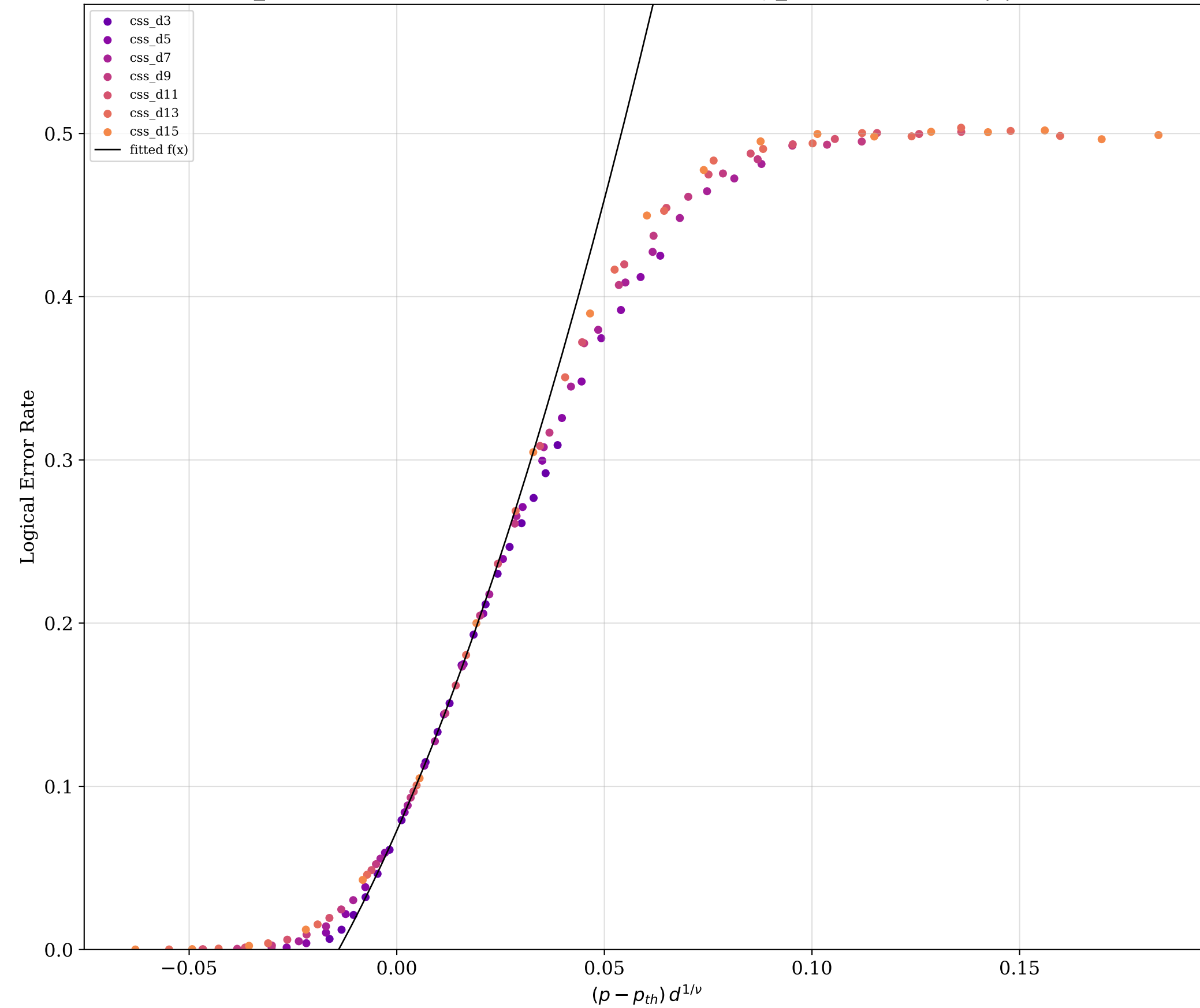
FSS data collapse ( \eta = 1 )
