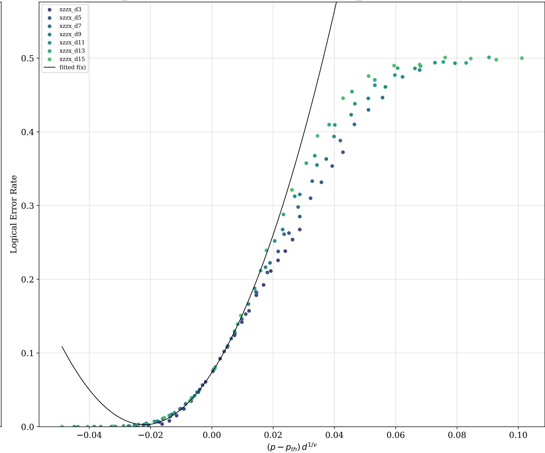
FSS data collapse ( \eta = 1 )
