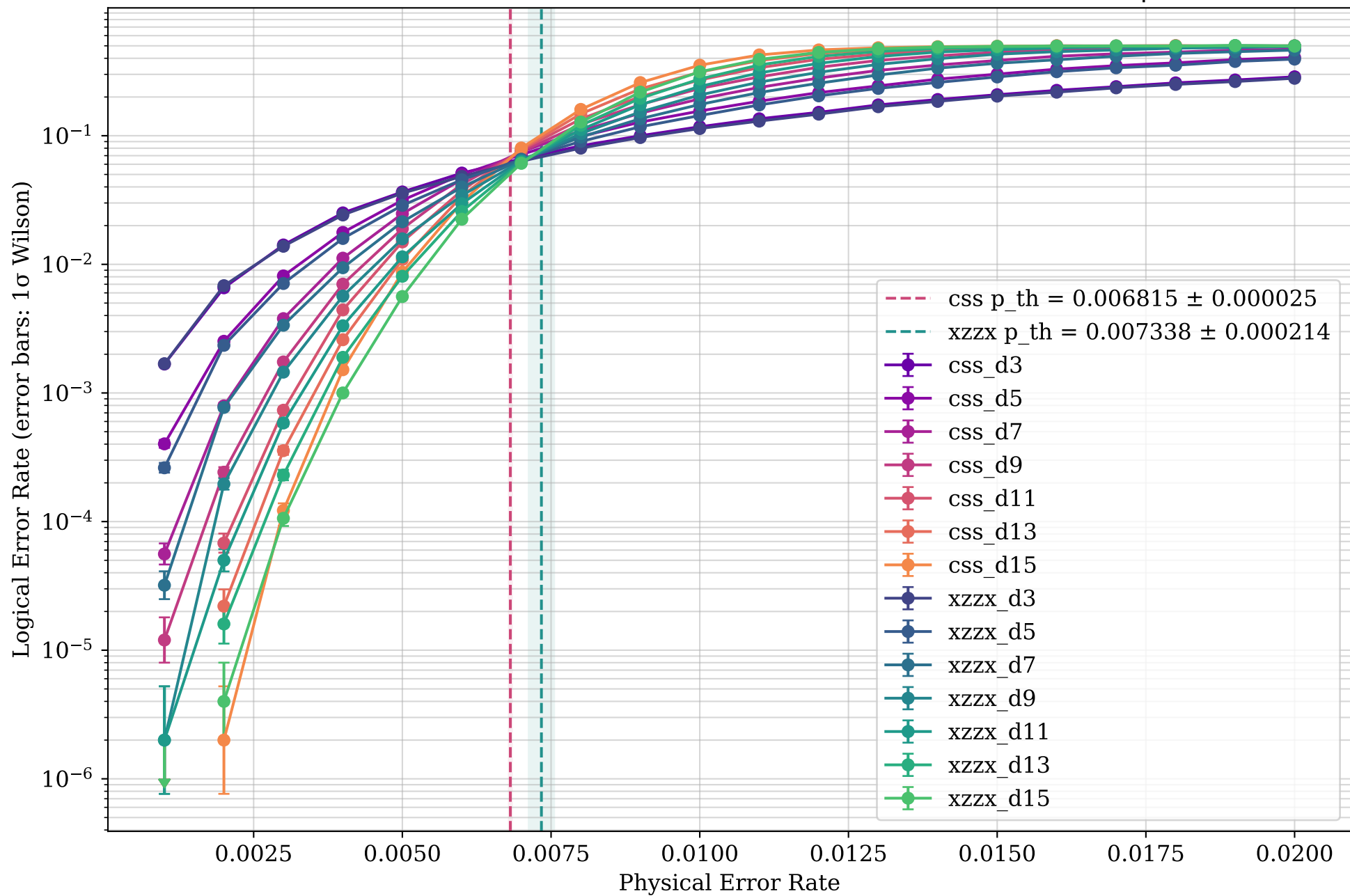
Rotated CSS Surface Code vs XZZX Code Simulation Results with \eta = 0.5
