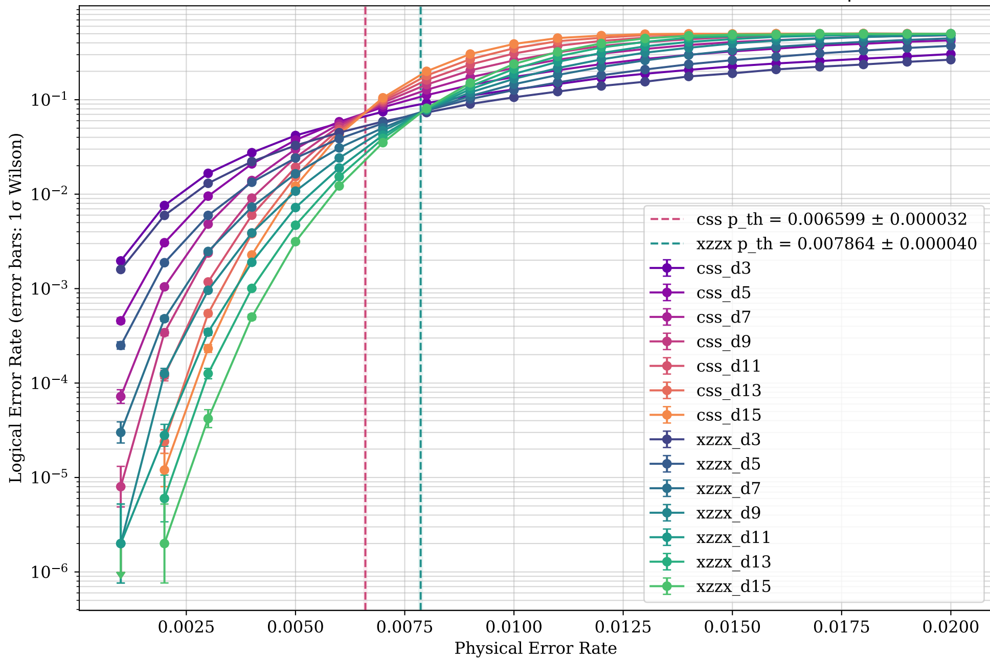
Rotated CSS Surface Code vs XZZX Code Simulation Results with \eta = 1
