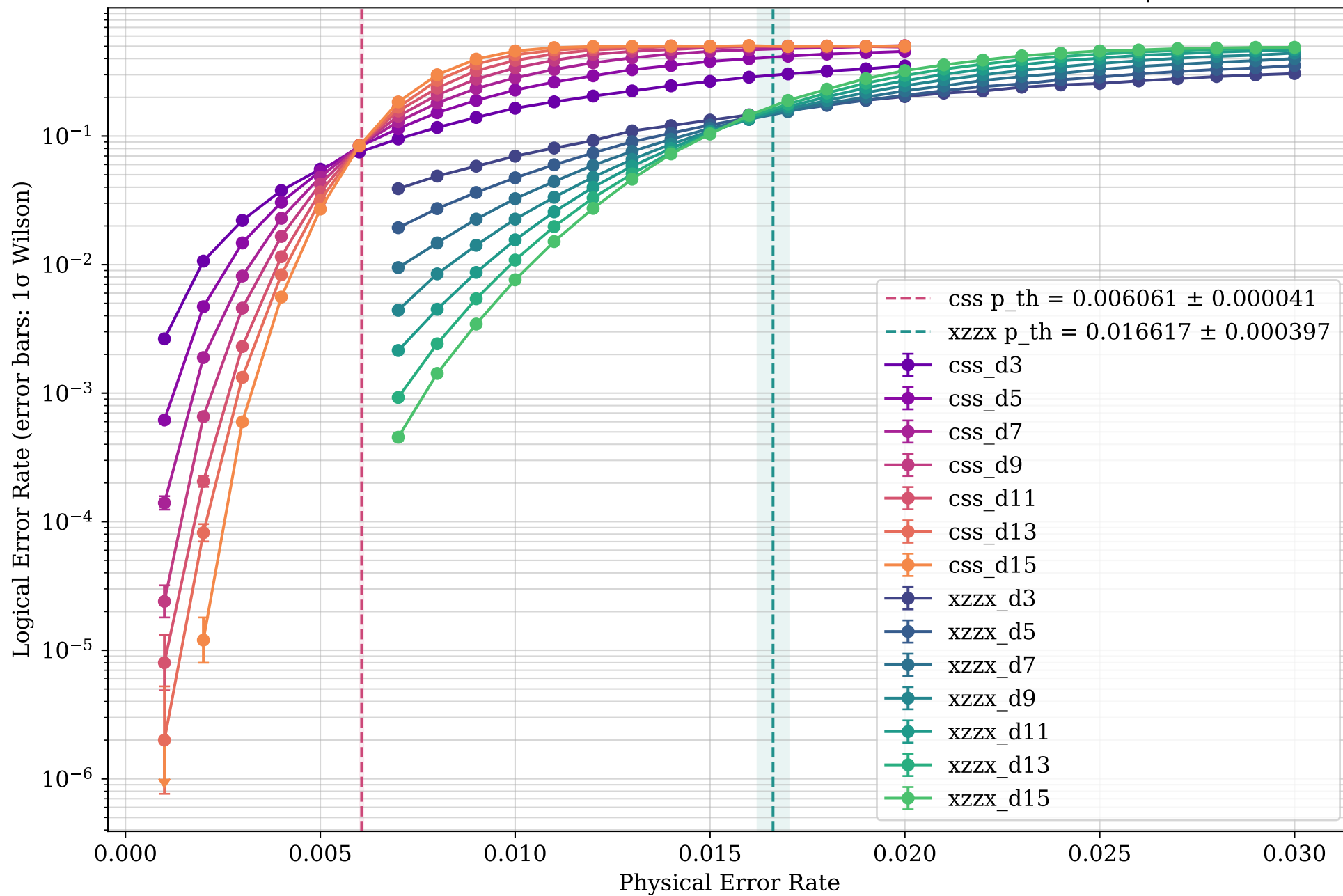
Rotated CSS Surface Code vs XZZX Code Simulation Results with \eta = 30
