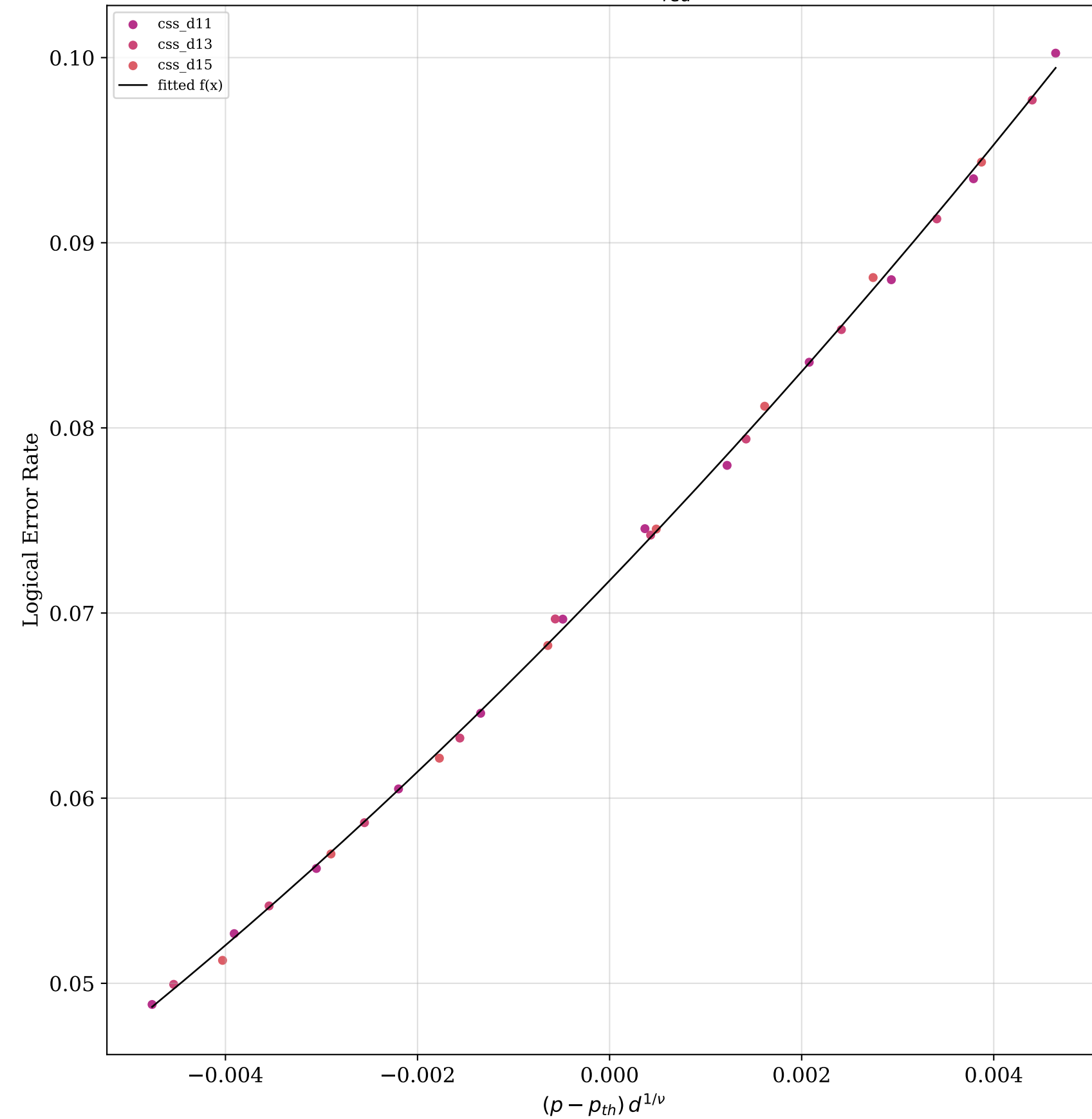
FSS data collapse ( \eta = 0.5 )
