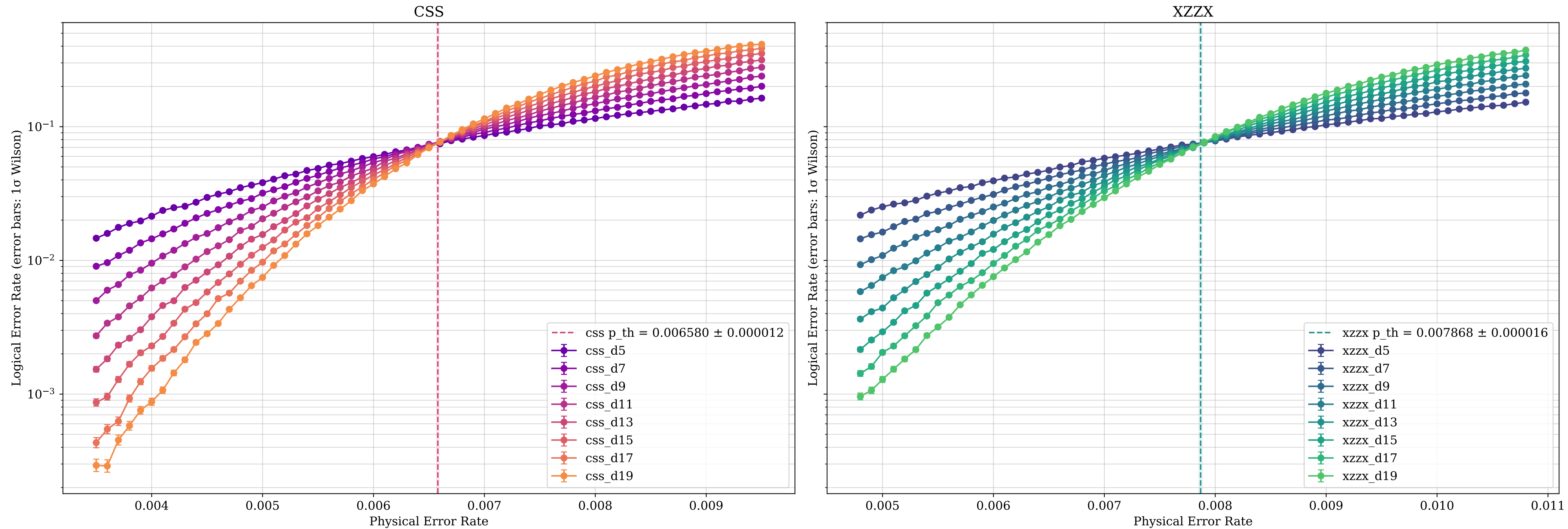
Rotated CSS Surface Code vs XZZX Code Simulation Results with \eta = 1
