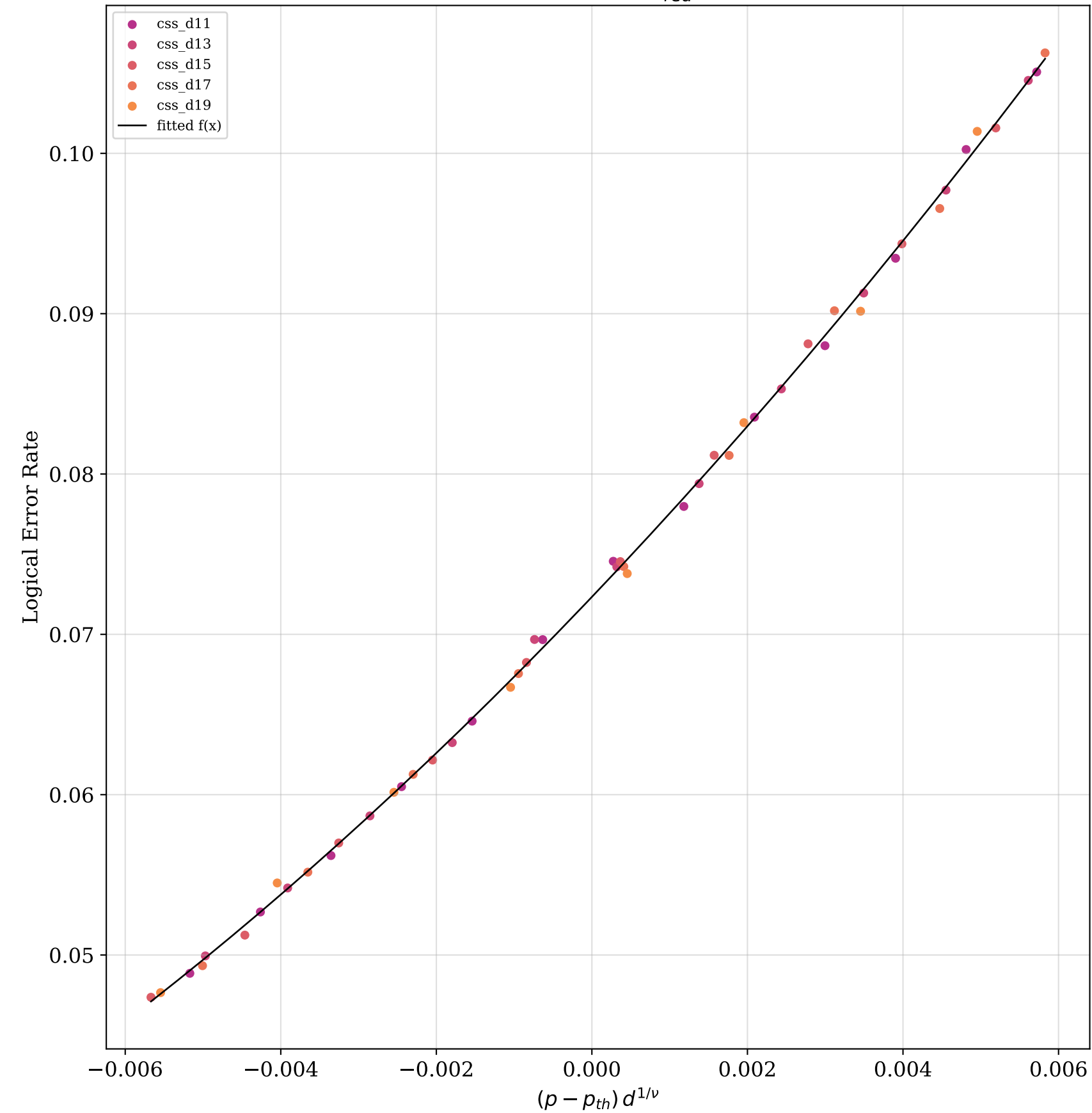
FSS data collapse ( \eta = 0.5 )
