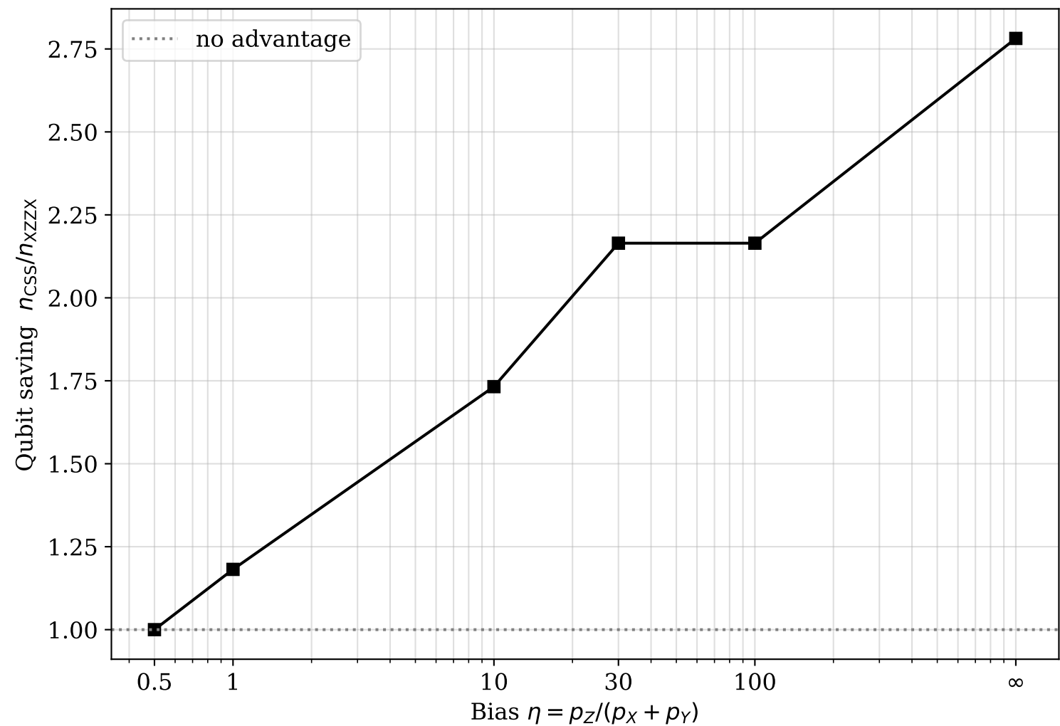
Physical-qubit cost vs bias (target per-cycle \varepsilon=1\text{e-}12 , physical p=0.001 ; memory only, square codes)
