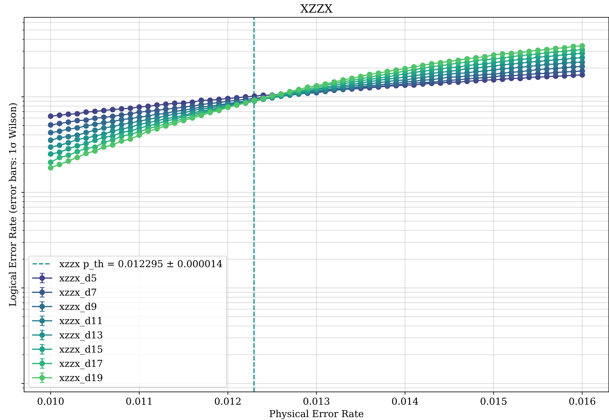
Rotated CSS Surface Code vs XZZX Code Simulation Results with \eta = 10
