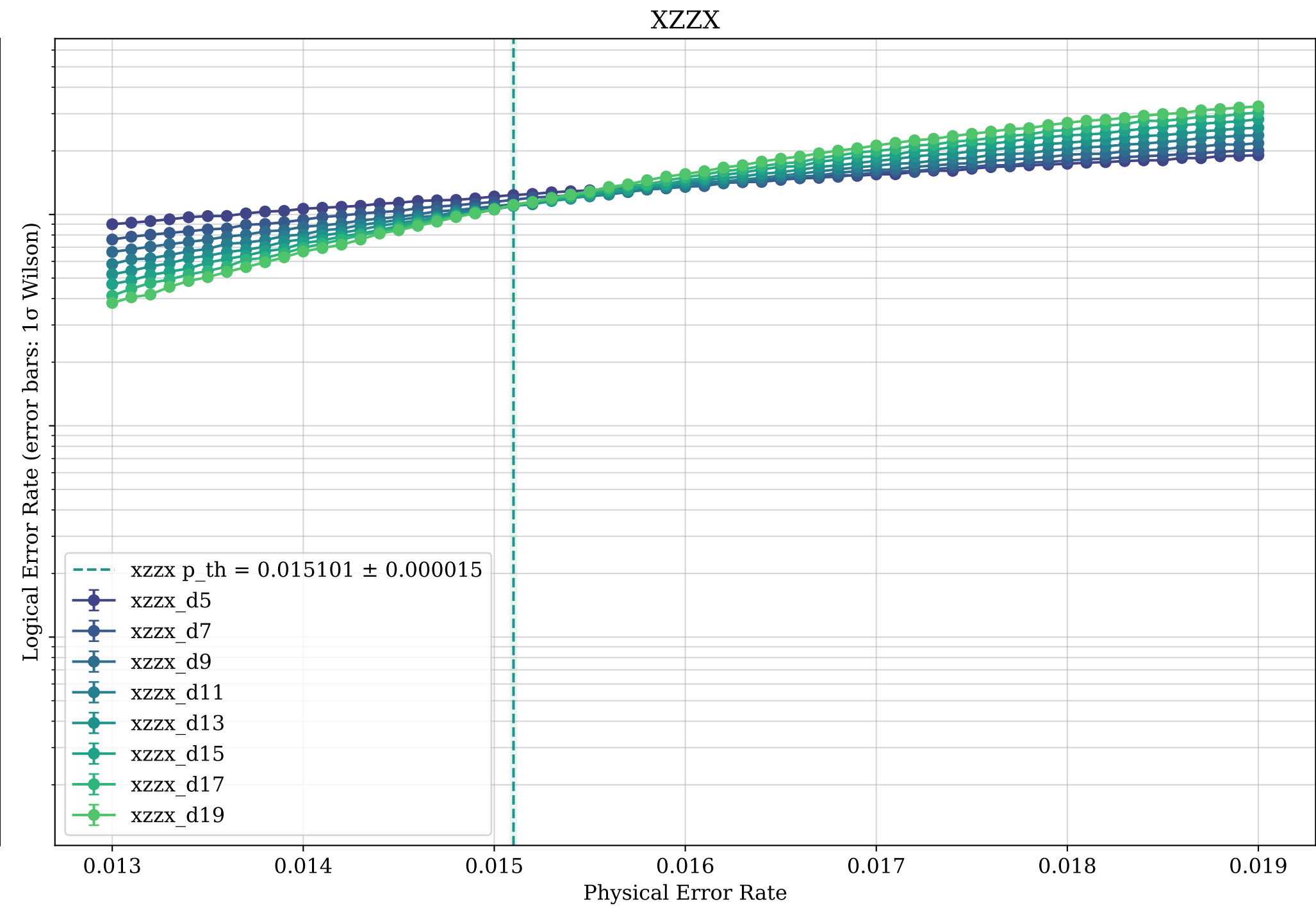
Rotated CSS Surface Code vs XZZX Code Simulation Results with \eta = 30
