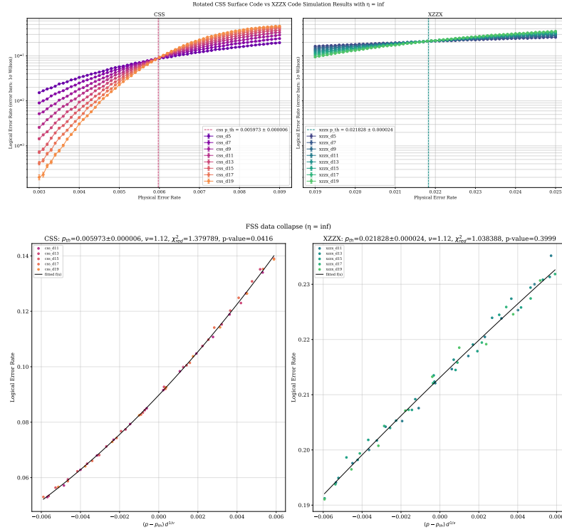
Figure A.6: Logical error rate (top) and FSS data collapse (bottom) at \eta \rightarrow \infty (pure dephasing).
