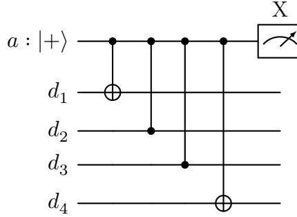
Figure 2.2: Syndrome-extraction gadget for an XZZX ancilla. The same prepare- |+\rangle , controlled-Pauli, measure- X gadget now mixes gate types: the schedule order yields CX , CZ , CZ , CX (i.e. XZZX ), with the X legs on one diagonal and the Z legs on the other.
