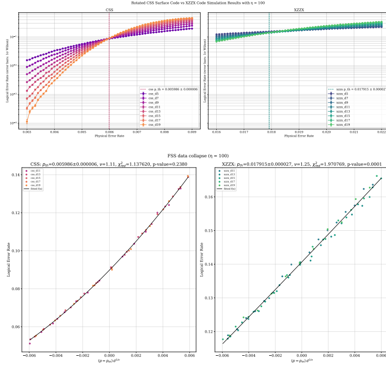
Figure A.5: Logical error rate (top) and FSS data collapse (bottom) at \eta = 100 .
