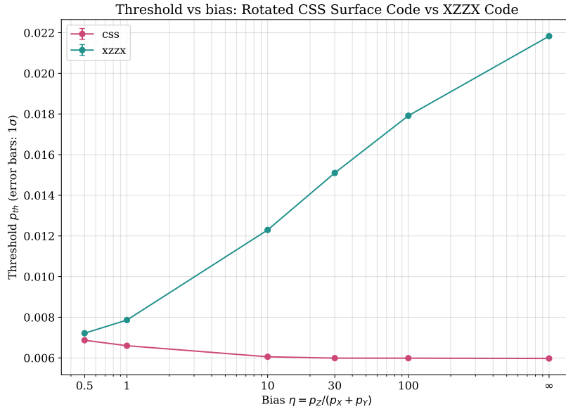
Figure 4.3: Fitted threshold p_{\text{th}} \pm \delta versus bias \eta (log-scaled, with \eta = \infty placed one decade past the largest finite bias) for both codes — the culminating CSS-versus-XZZX comparison. The XZZX threshold rises monotonically with bias while the CSS threshold stays essentially flat.
