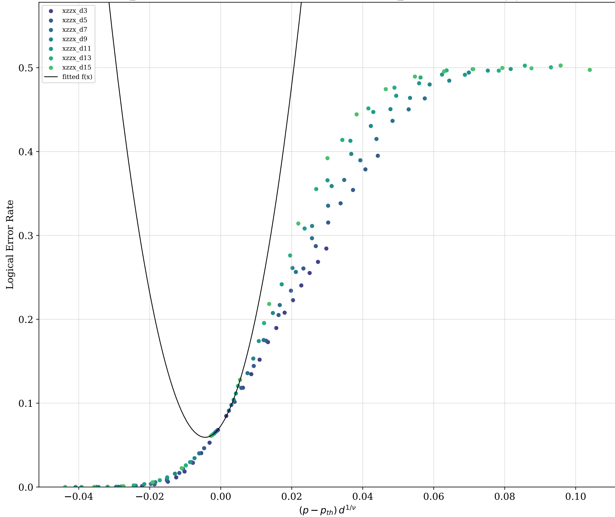
FSS data collapse ( \eta = 0.5 )
