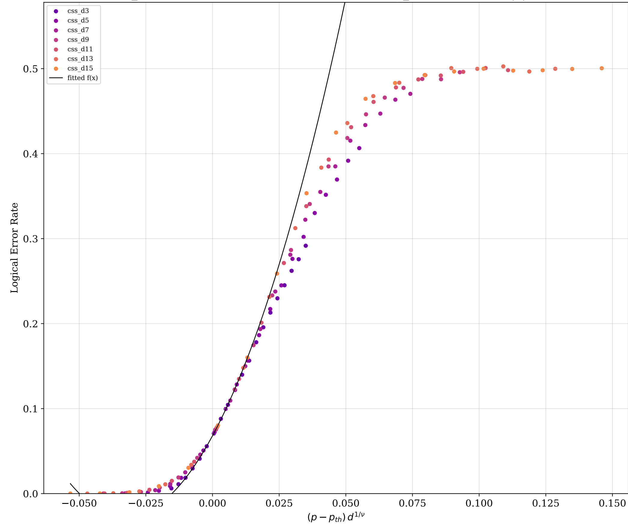
FSS data collapse ( \eta = 0.5 )
