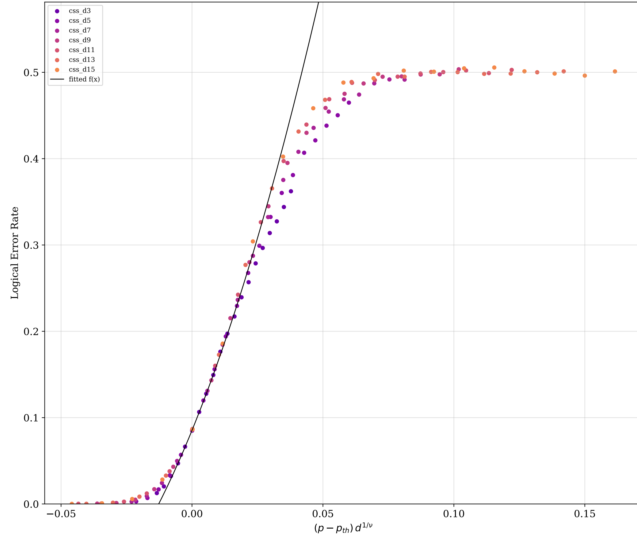
FSS data collapse ( \eta = 100 )
