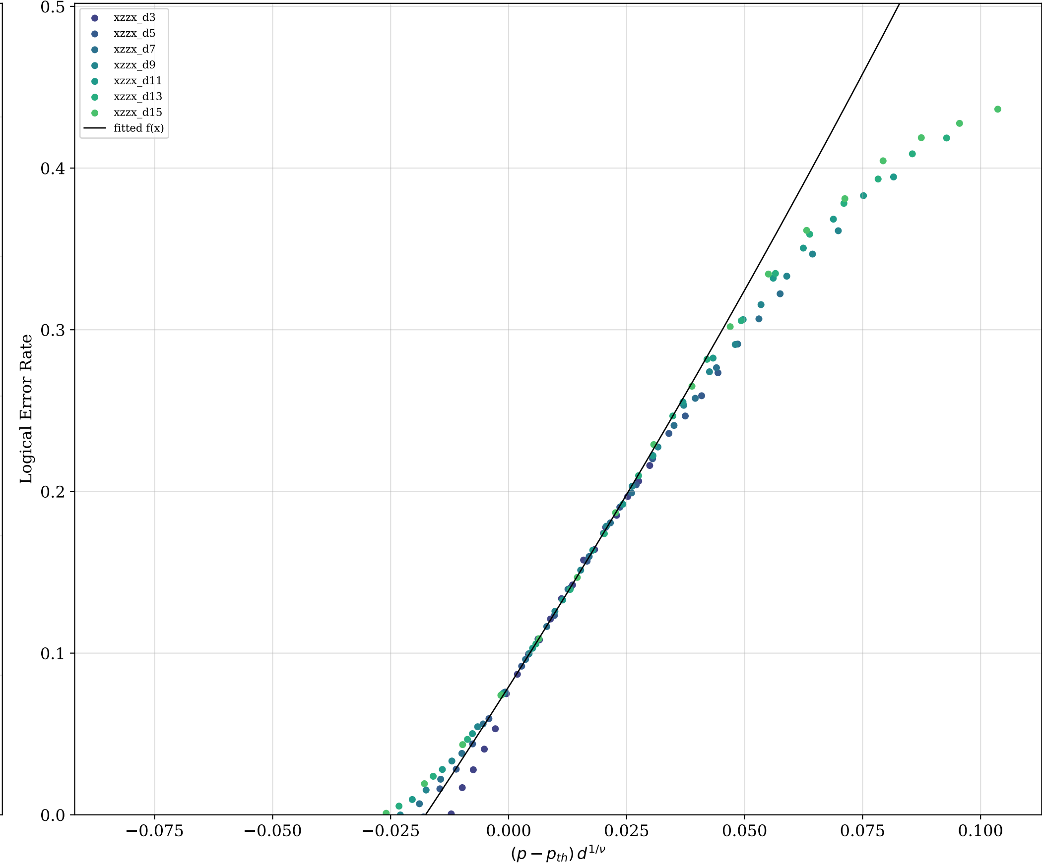
FSS data collapse ( \eta = 100 )
