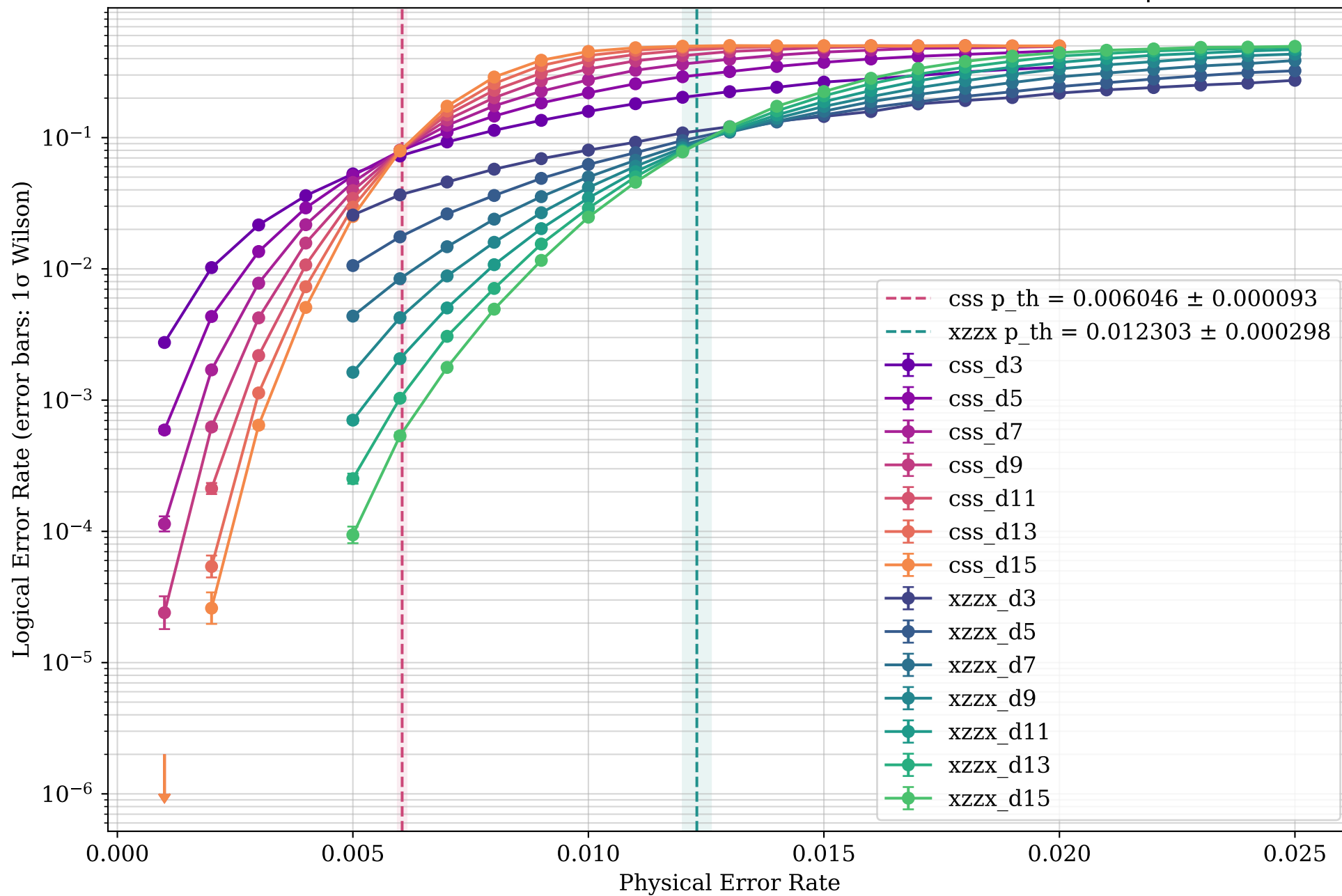
Rotated CSS Surface Code vs XZZX Code Simulation Results with \eta = 10
