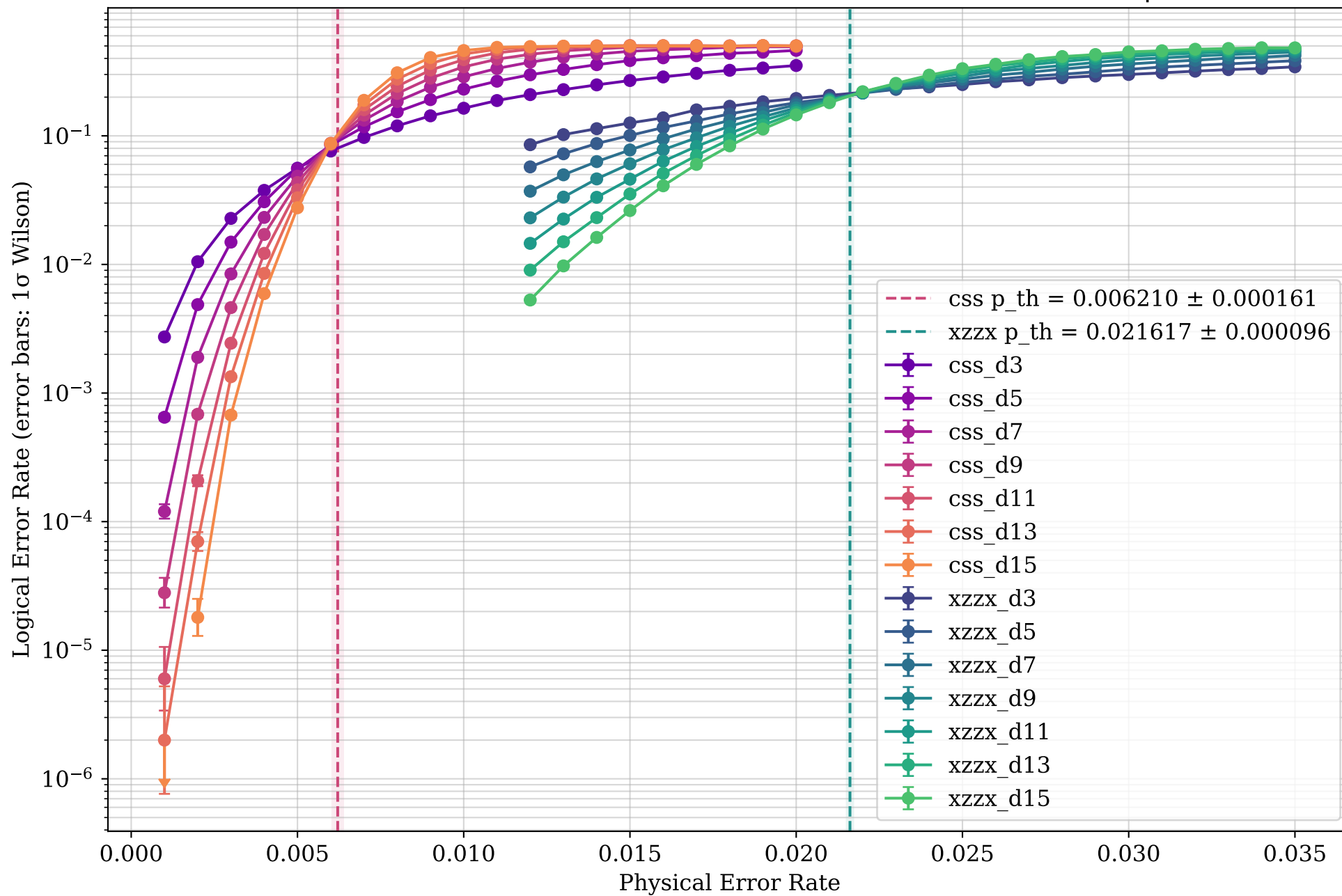
Rotated CSS Surface Code vs XZZX Code Simulation Results with \eta = \infty
