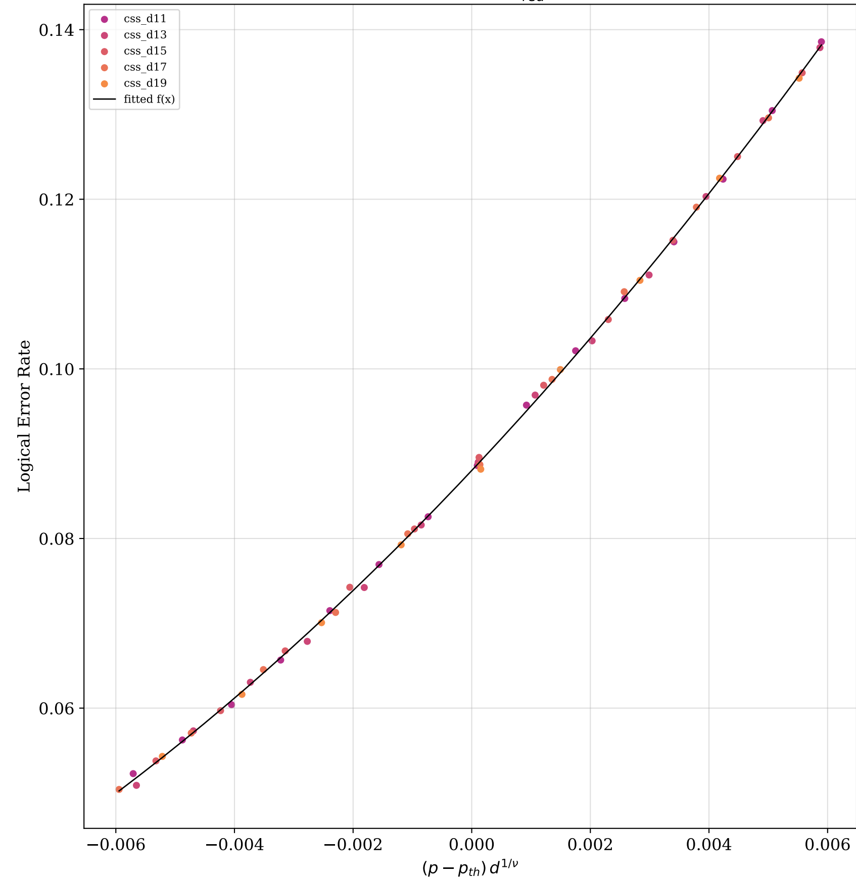
FSS data collapse ( \eta = 30 )
