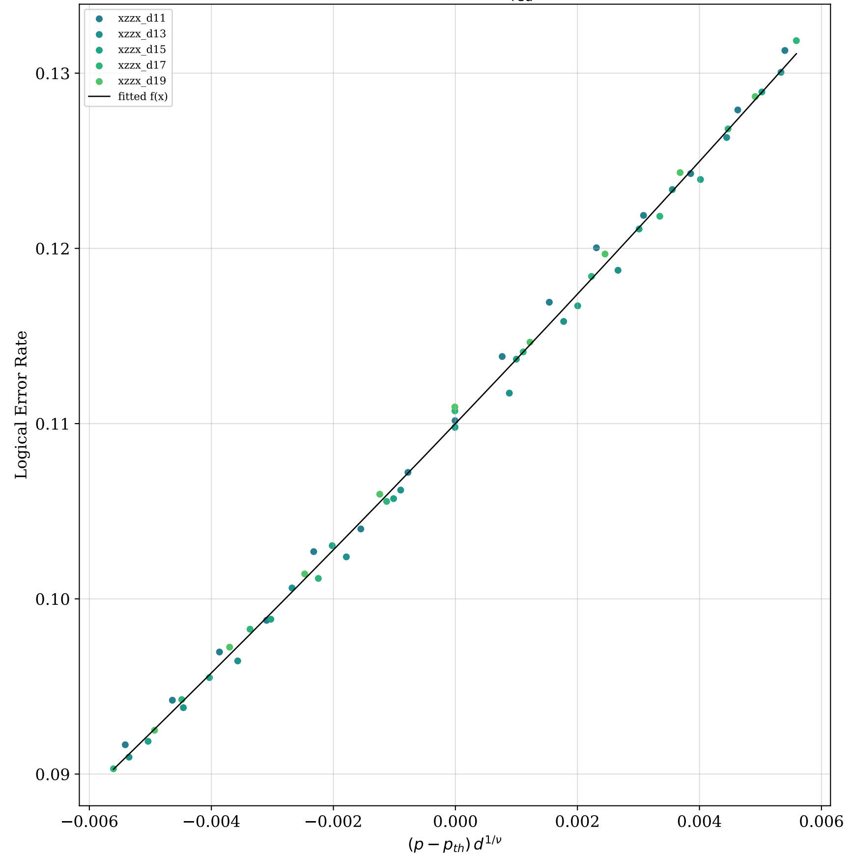
FSS data collapse ( \eta = 30 )
