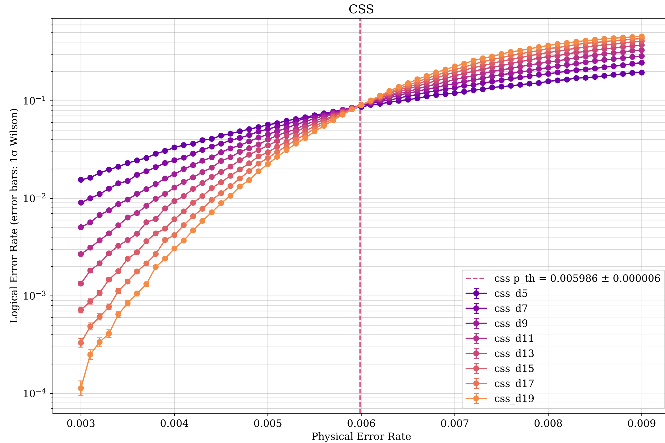
Rotated CSS Surface Code vs XZZX Code Simulation Results with \eta = 100
