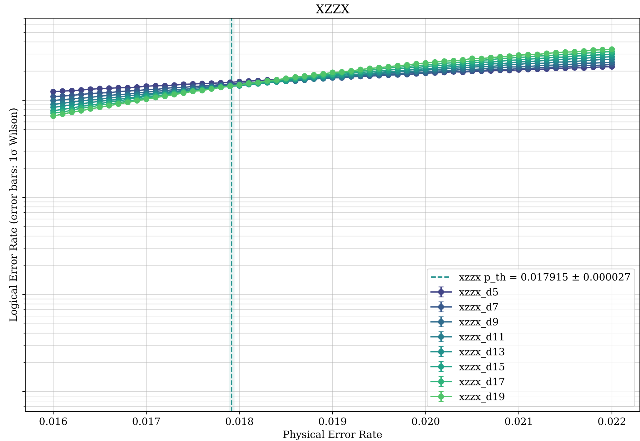
Rotated CSS Surface Code vs XZZX Code Simulation Results with \eta = 100
