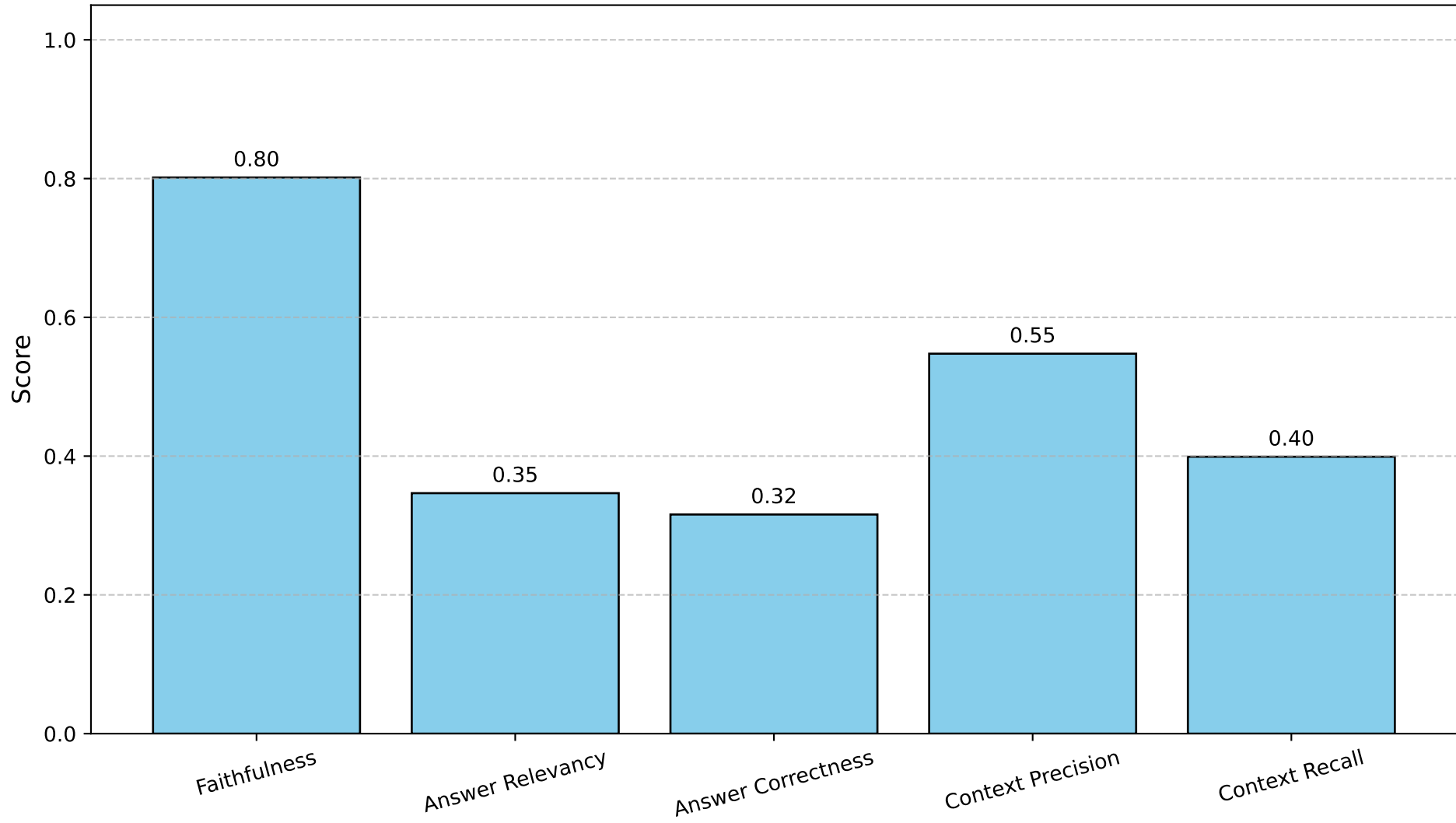
Average RAG Evaluation Metrics for Baseline System (25 Queries)
