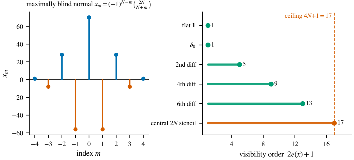
Figure 3: The finite prime-edge uncertainty ceiling at N = 4 . Left: the unique maximally blind normal, the centered finite-difference stencil x_m = (-1)^{N-m} \binom{2N}{N+m} . Right: the visibility order 2e(x) + 1 of a family of even normals climbs by 4 with each additional vanishing moment and is capped at 4N + 1 = 17 , attained only by the central-difference stencil.
