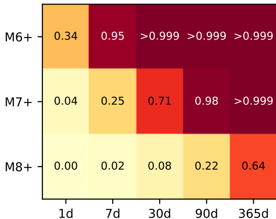
Prospective: 0 to +w days
