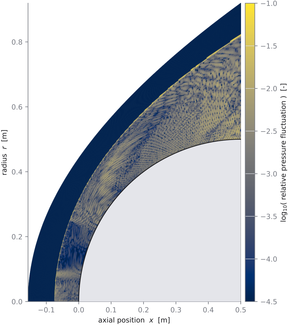
(c) sphere_M6_fine_Co0p1, max Co 0.1 (of record) |p(it 110,000) – p(it 105,000)| / p, saved fields 5,000 it apart max 1.2\text{e-}01 · median in the shock layer 9.0\text{e-}04
