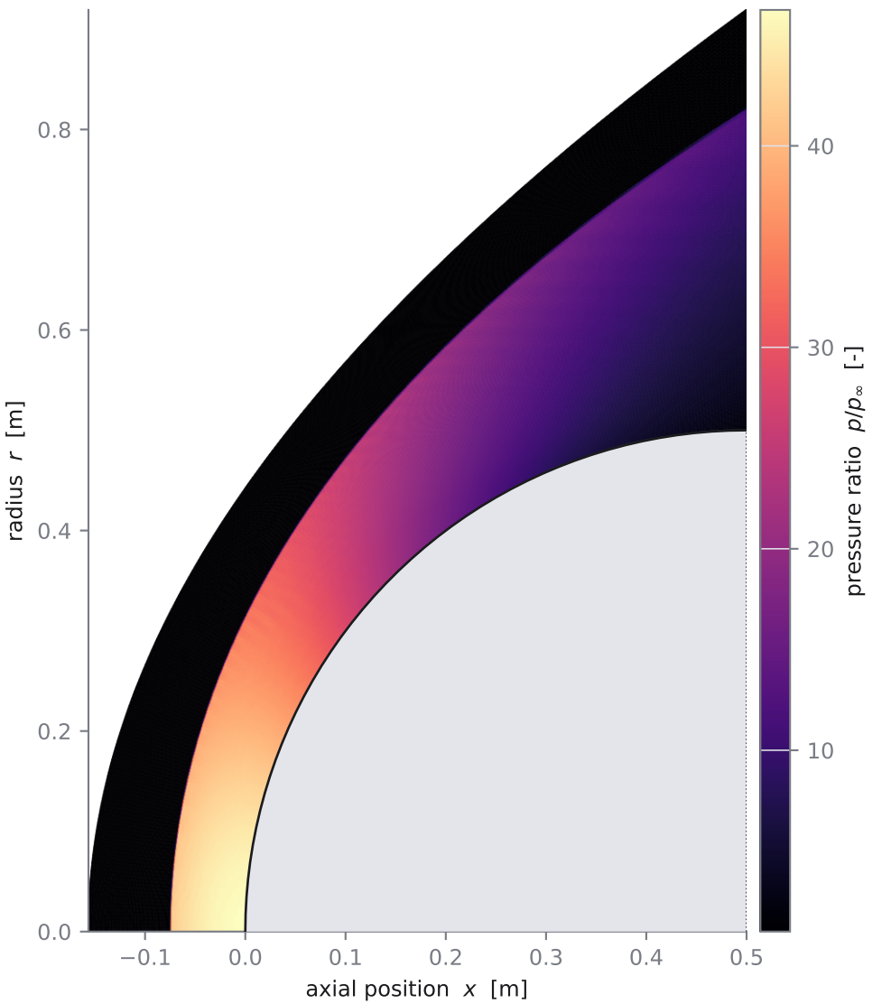
(d) sphere_M6_fine_Co0p1 p/p ∞ at it 110,000 (the field of record)
