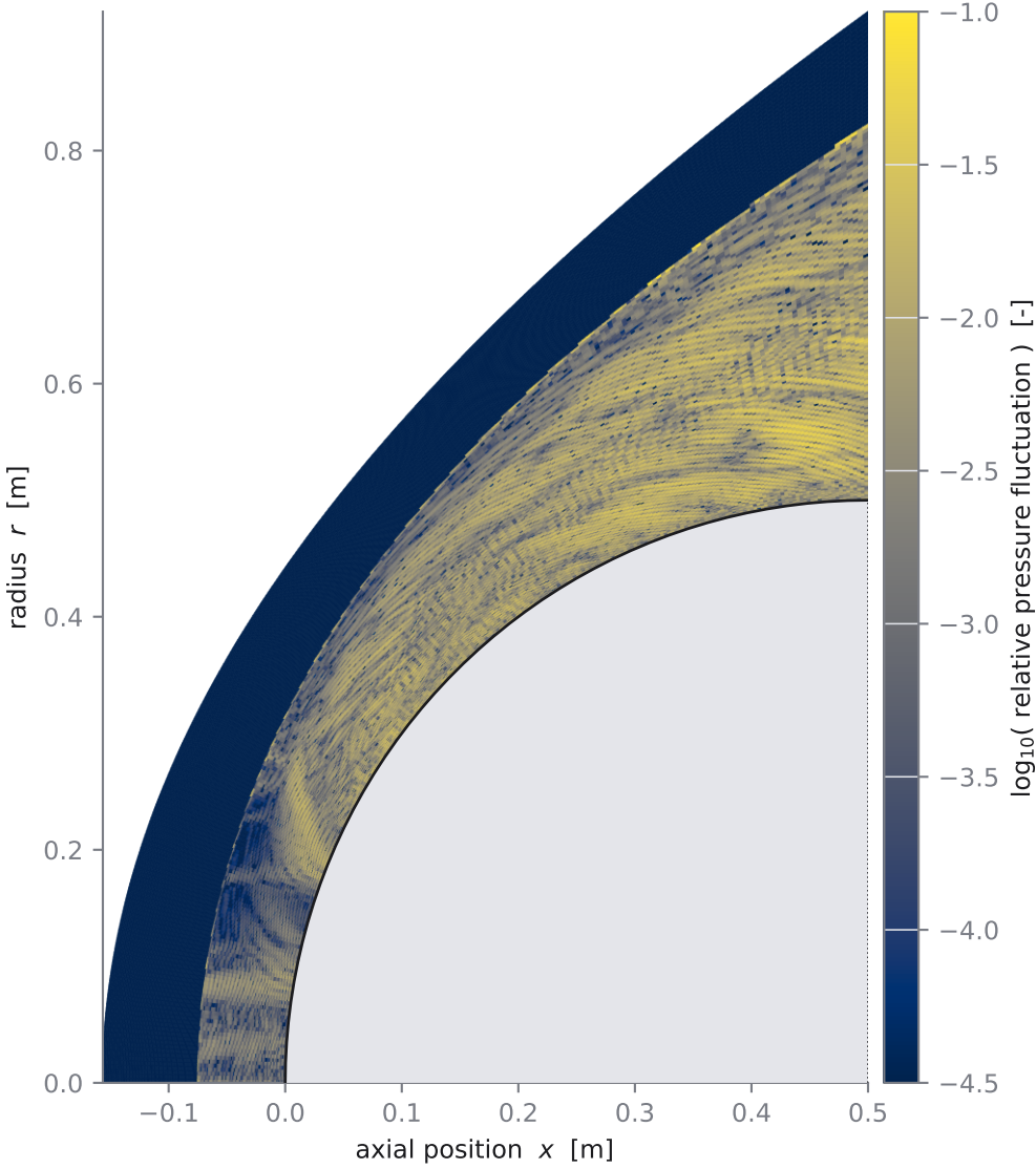
(b) sphere_M6_fine, max Co 0.2 |p(it 100,000) – p(it 80,000)| / p, saved fields 20,000 it apart max 1.1\text{e-}01 · median in the shock layer 3.6\text{e-}03
