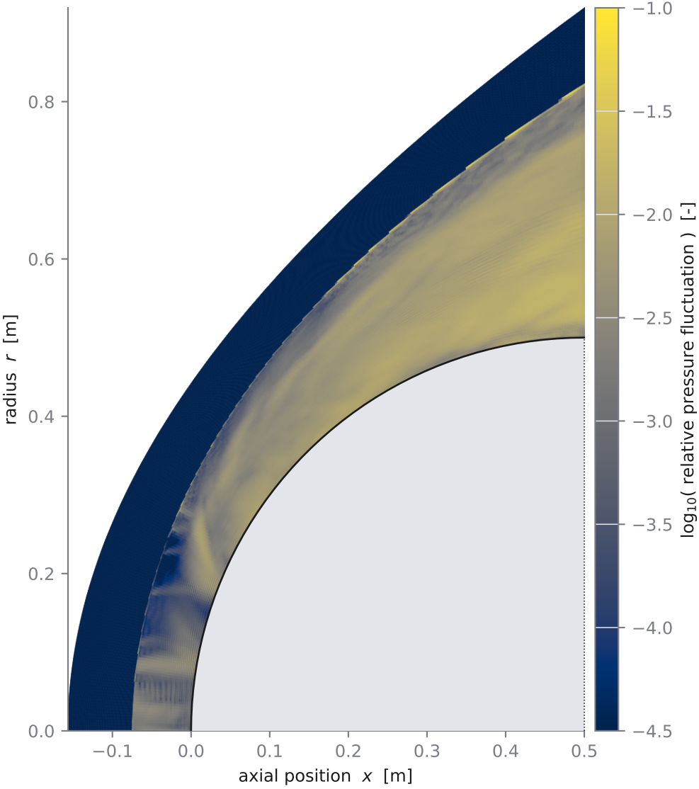
(a) sphere_M6_fine_cyclediag, max Co 0.2 rms of p over 100 snapshots, it 100,002–100,200 every 2 max 4.8\text{e-}02 · median in the shock layer 4.2\text{e-}03
