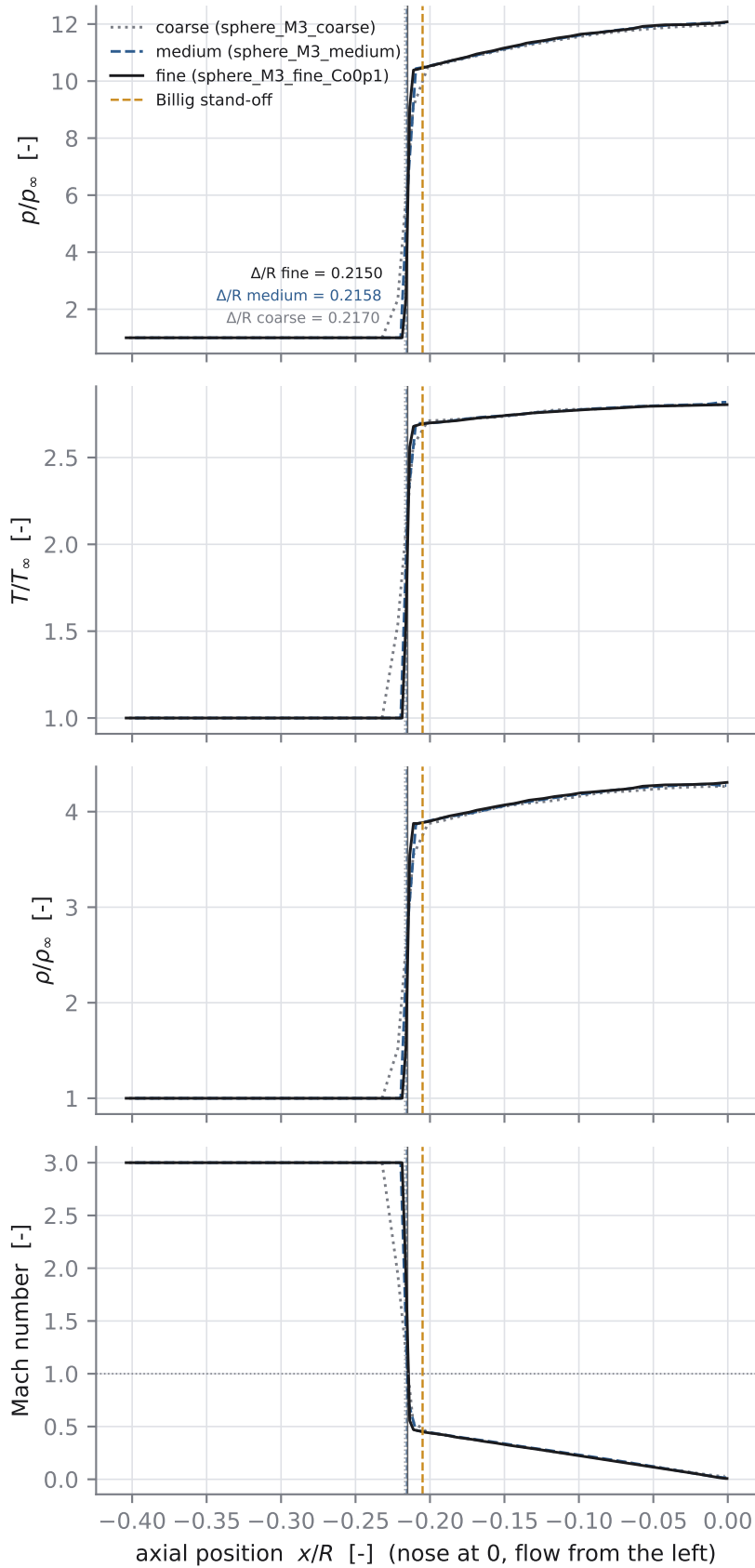
sphere, M_\infty = 3 : stagnation line (axis, r = 0 )
