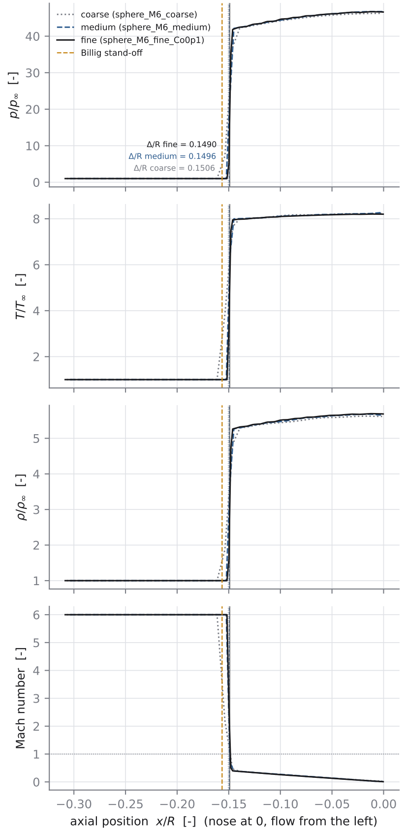
sphere, M_\infty = 6 : stagnation line (axis, r = 0 )
