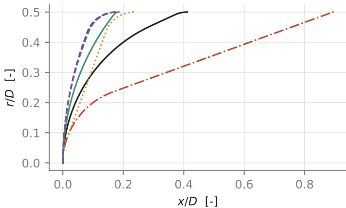
forebody outlines, M_\infty = 20
