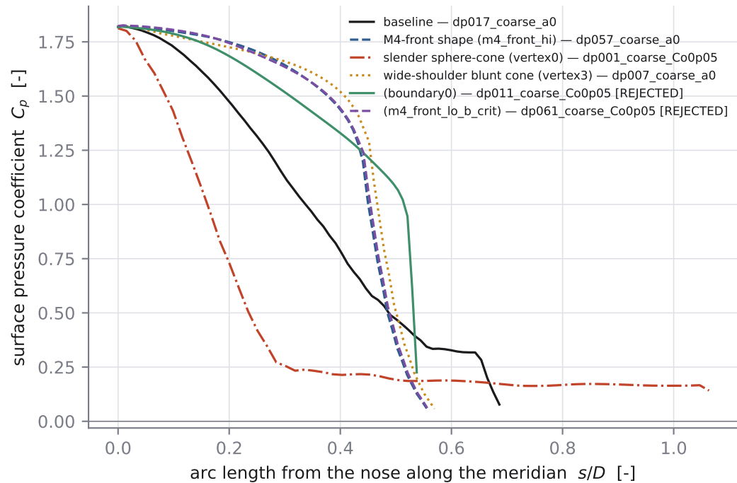
C_p along the forebody, M_\infty = 20 , coarse mesh
