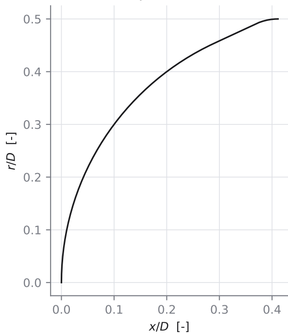
forebody outlines, M_\infty = 6
