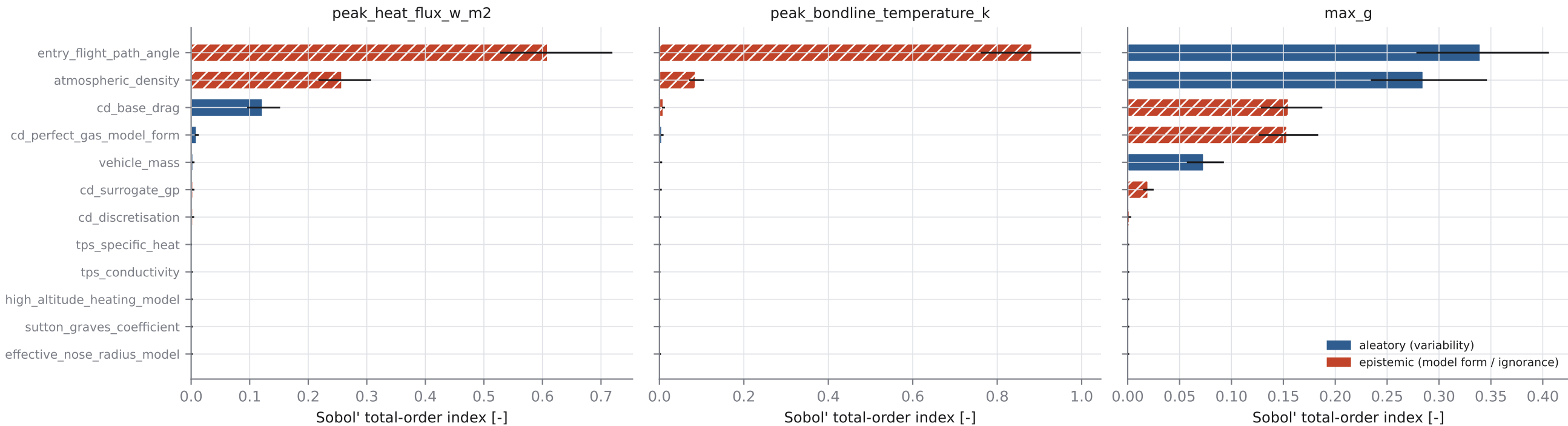
Variance attribution on design 'baseline' (bars: total order; lines: 95% bootstrap interval)
