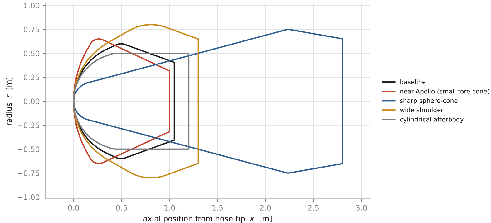
Capsule geometry family across the parametric bounds
