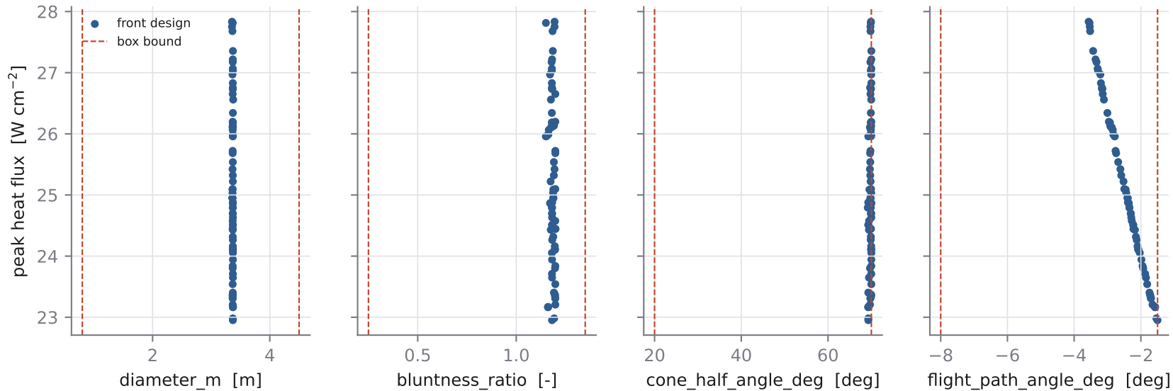
AETHER M4 · run M4-OPT-20260920T205252Z · DOE M4-DOE-20260920T204844Z · FIDELITY 1 (aero model: cfd_surface_v2). Each combined-front design's value of each active variable. Points stacked on a dashed line are parked on a box bound (see the exploit audit).
