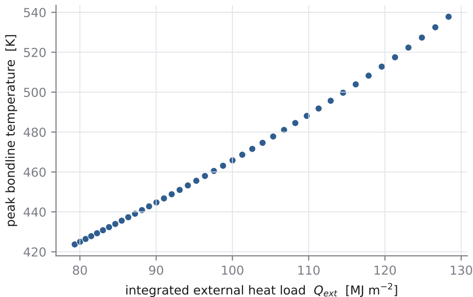
Bondline temperature tracks the integral, not the peak
