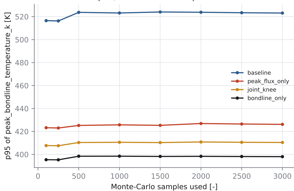
p95, with 95% bootstrap interval
