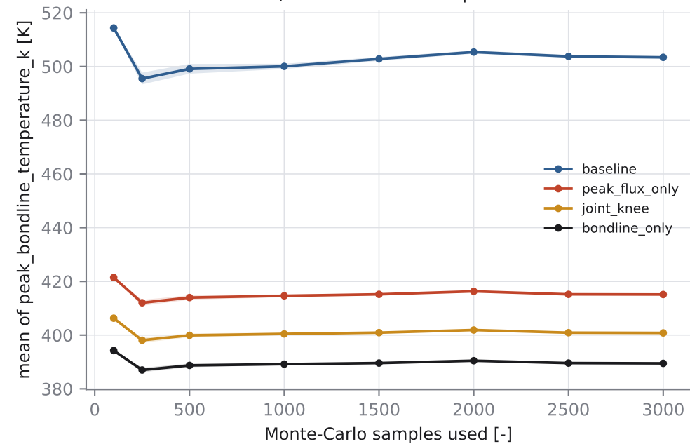
mean, with 95% bootstrap interval
