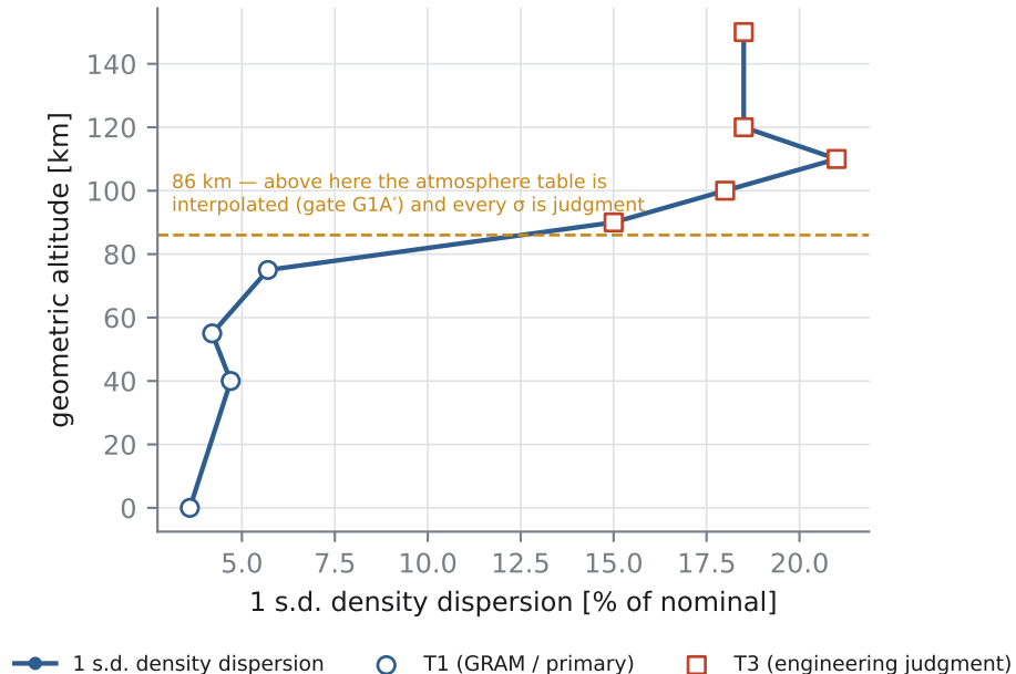
Atmospheric density dispersion
