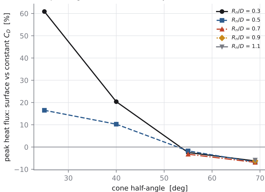
Shape acting THROUGH DRAG (zero by construction at constant C_D )
