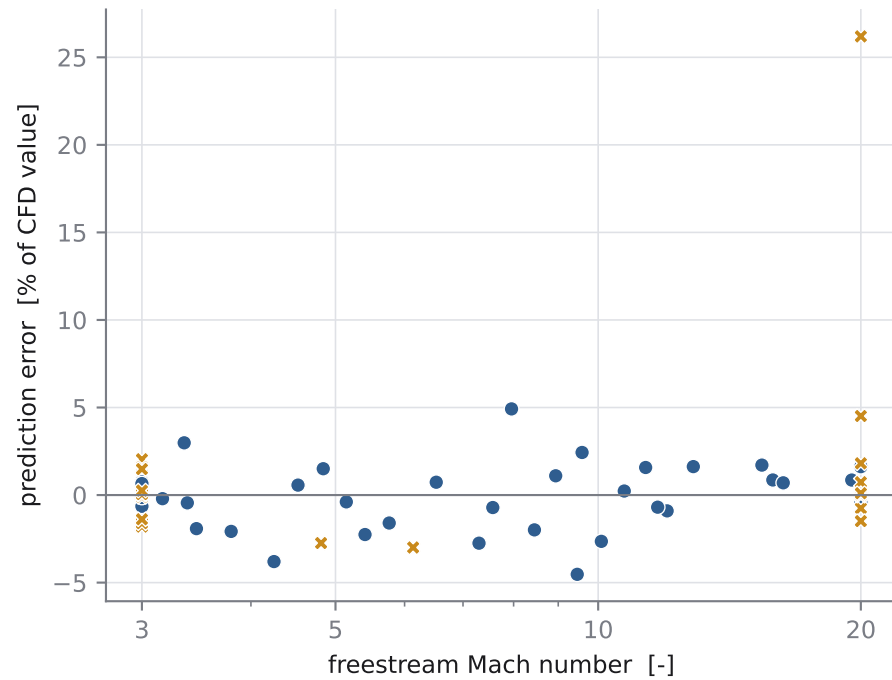
out-of-fold error against Mach
