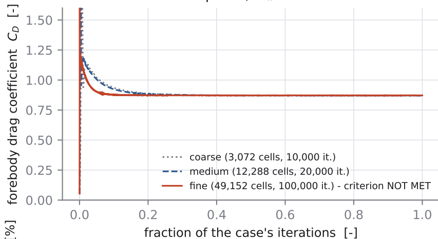
sphere, M_\infty = 6
