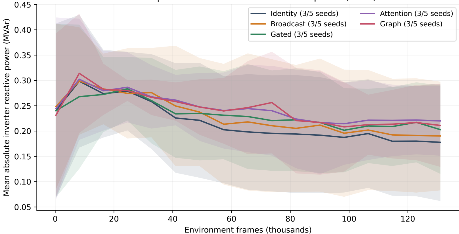
MAPDN | Mean absolute inverter reactive power (MVar)
