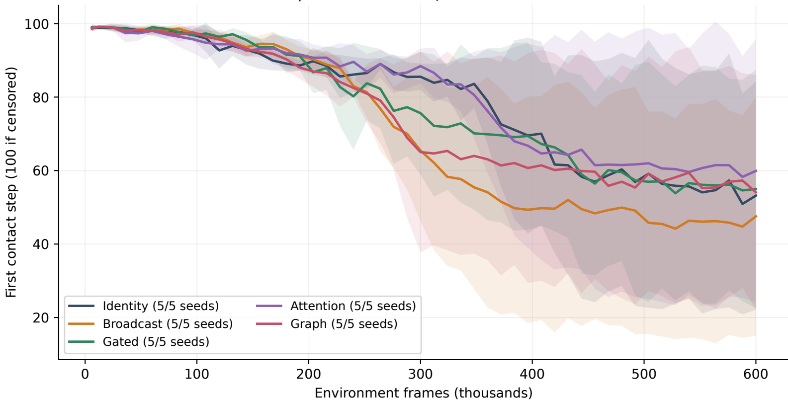
PCP | First contact step (100 if censored)
