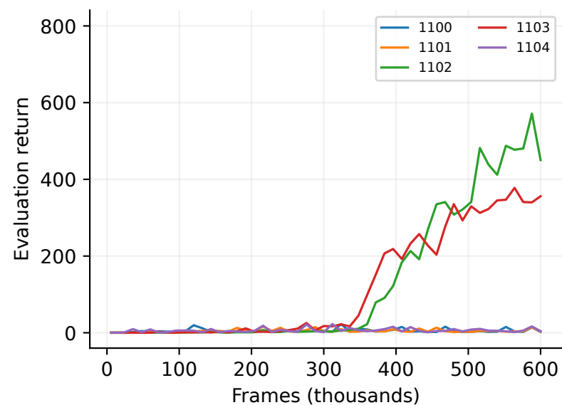
Attention
