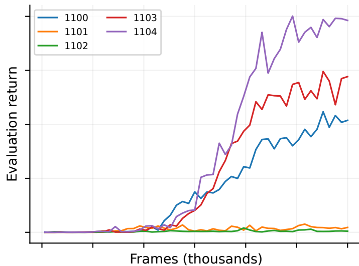
Graph
