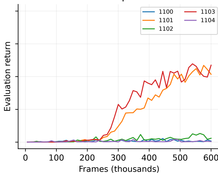
Graph
