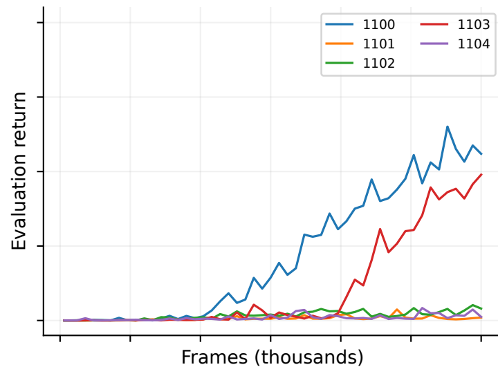
Gated
