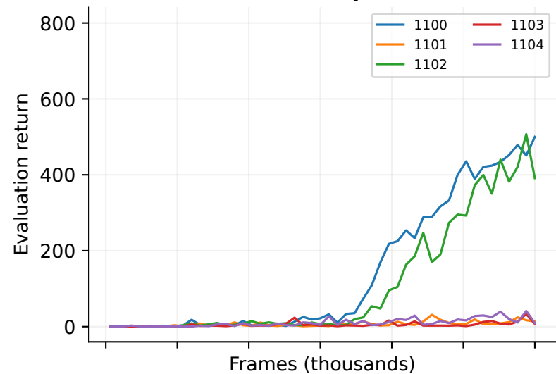
Attention
