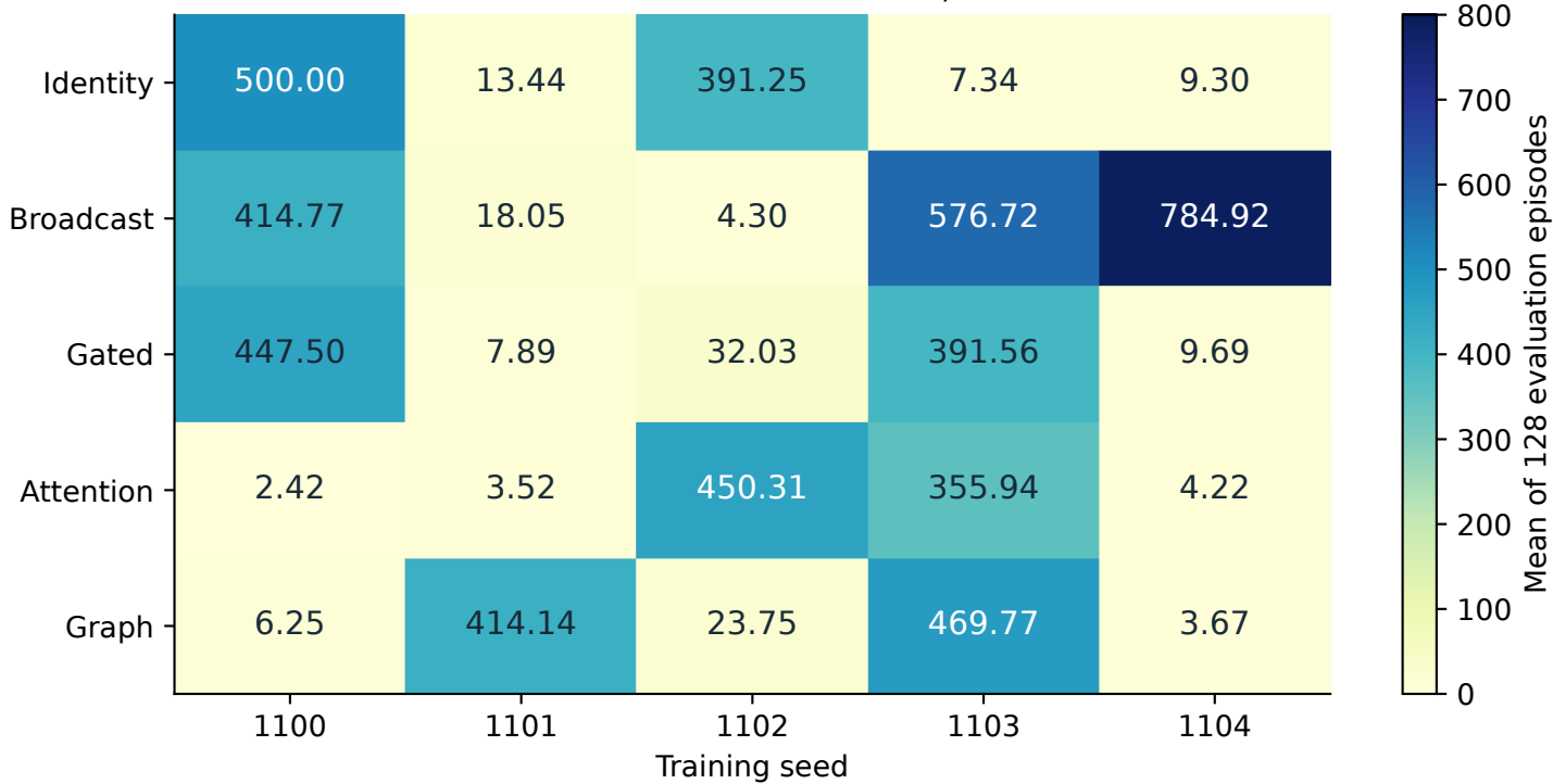
PCP final evaluation return at 600,000 frames
