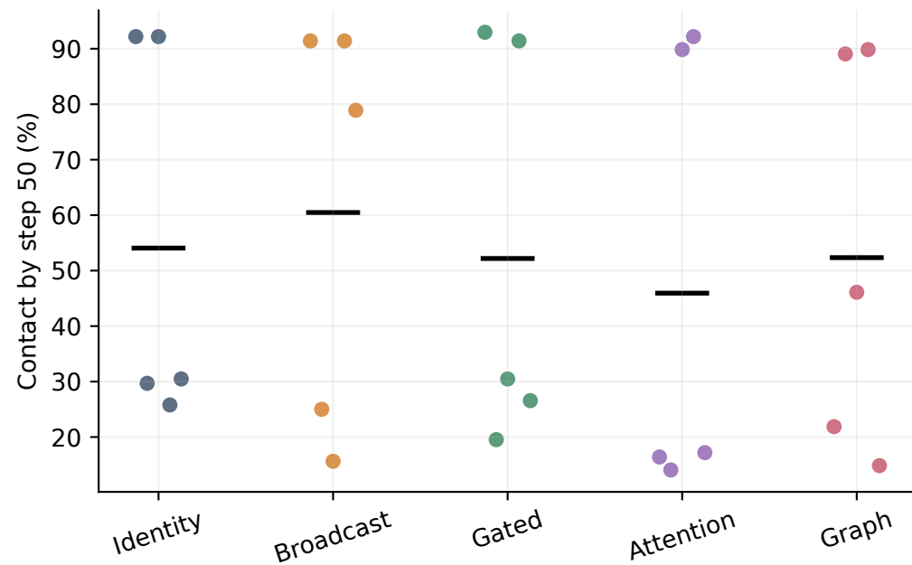
PCP final task outcomes: dots = training seeds; black marks = seed means
