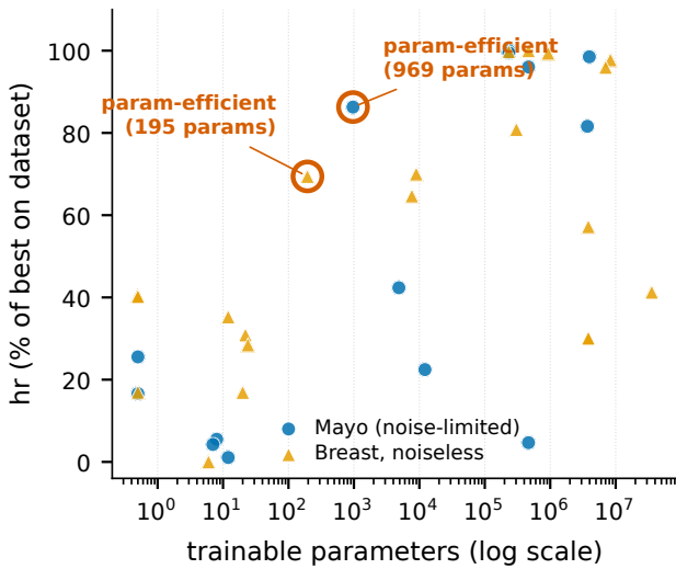
FIGURE 2 | Accuracy versus parameter count for both datasets (Mayo and breast noiseless). To overlay the two different hr scales, each solver’s hr is normalized to the percent of the best hr reached on its own board. The agent’s compact recombination solver is ringed: 969 parameters on Mayo, 195 on breast. It reaches the top accuracy tier at \sim 1\text{--}2\% of the parameters of the variational network.
